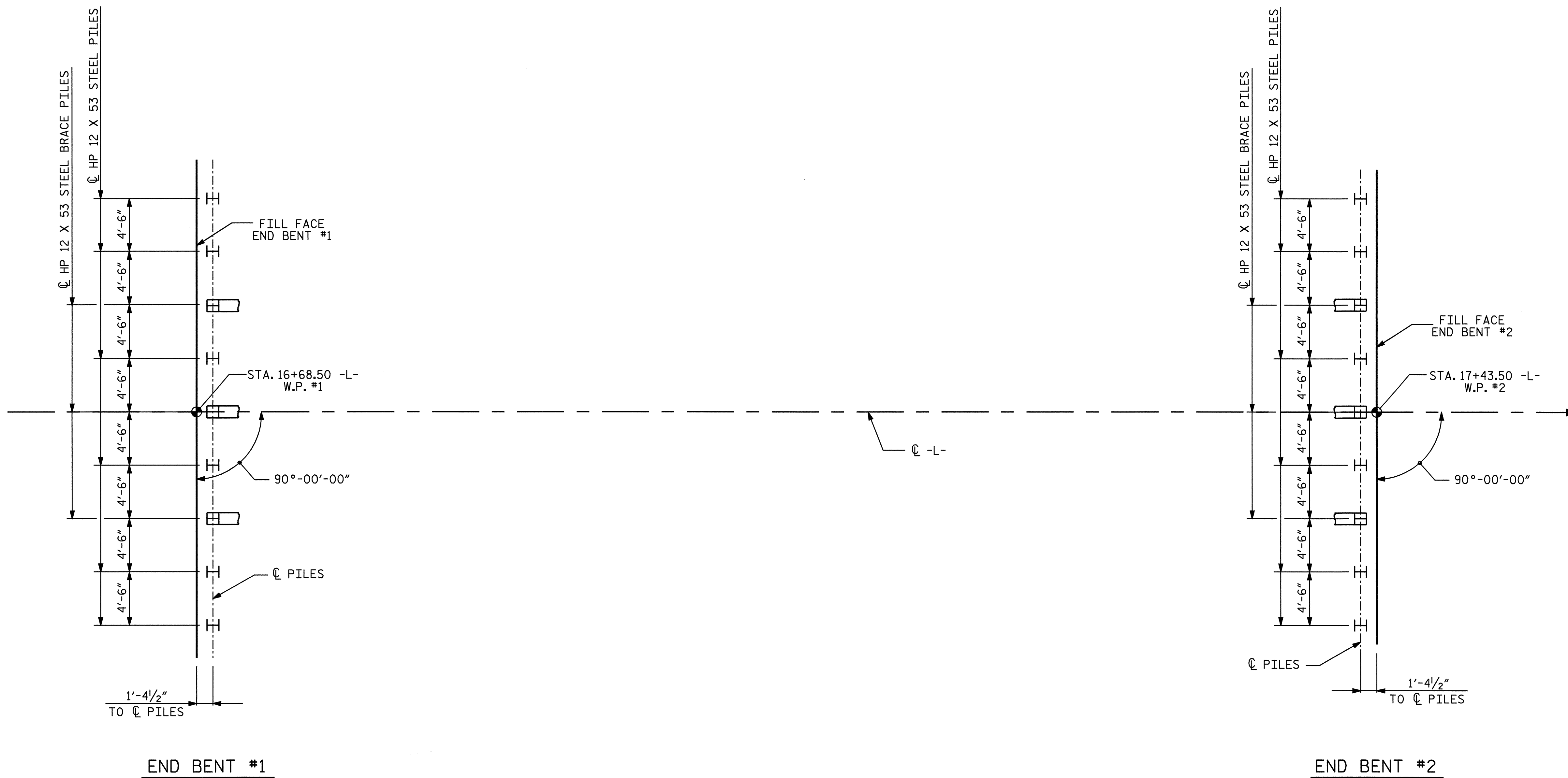
FOUNDATION LAYOUT HP 12 X 53 STEEL BRACE PILES ARE BATTERED 3:12 DIMENSIONS LOCATING PILES ARE SHOWN TO THE PILE CENTERLINE
