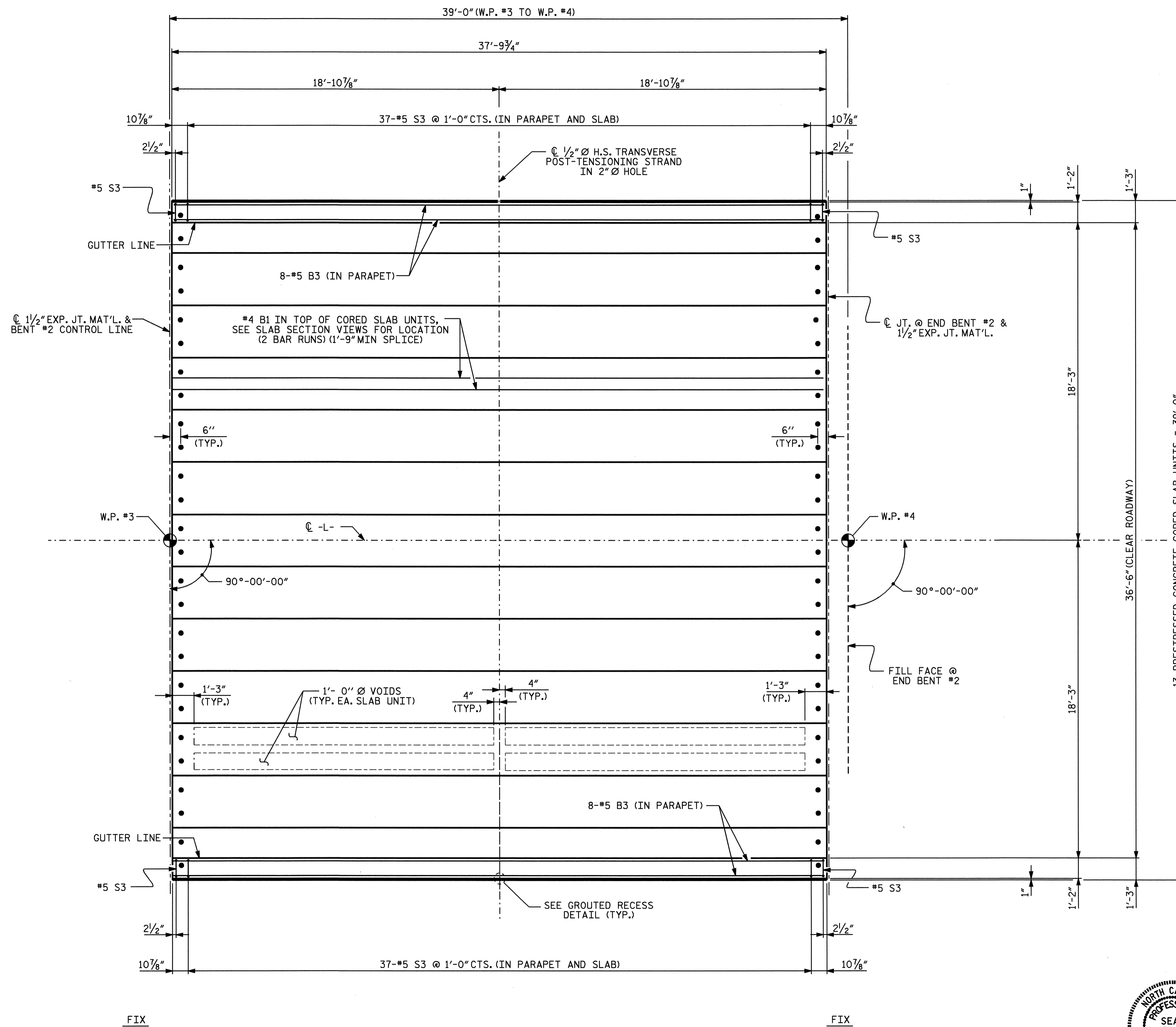
PLAN OF SPAN C
