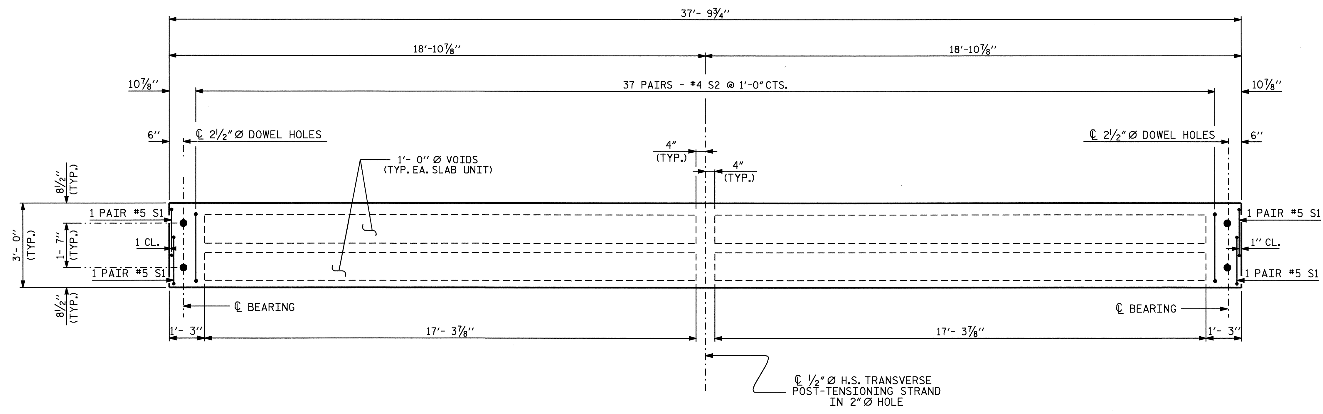
PLAN OF INTERIOR CORED SLAB UNIT (SPANS A & C)
