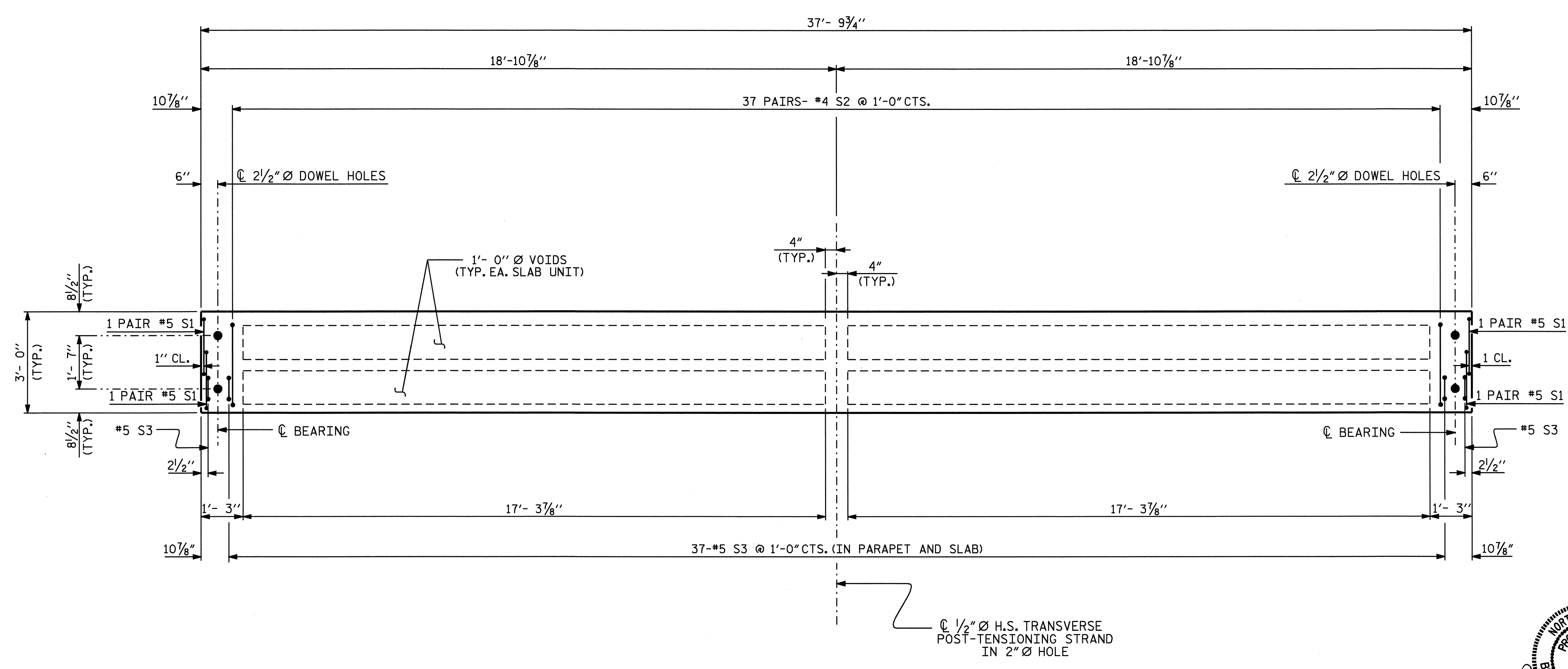
PLAN OF EXTERIOR CORED SLAB UNIT (SPANS A & C)
