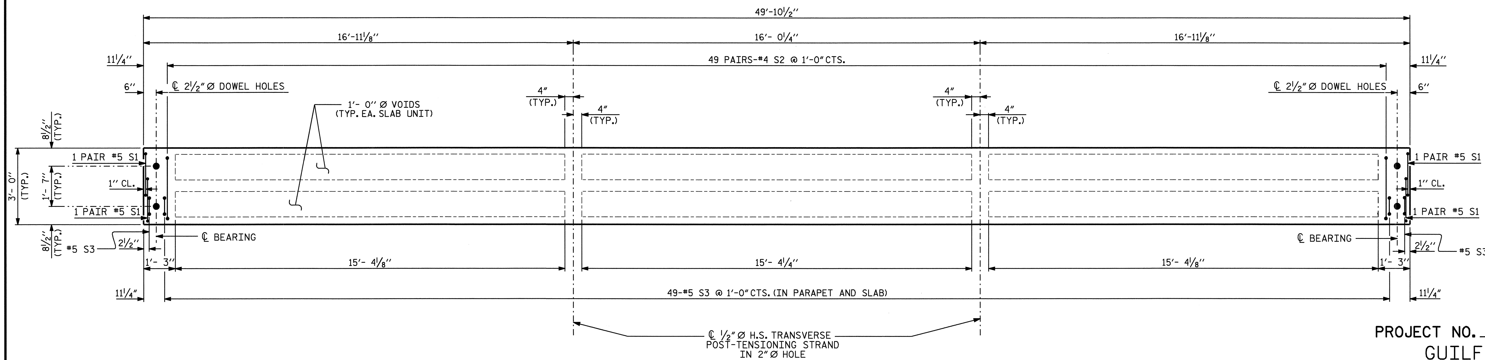
PLAN OF EXTERIOR CORED SLAB UNIT (SPAN B)
