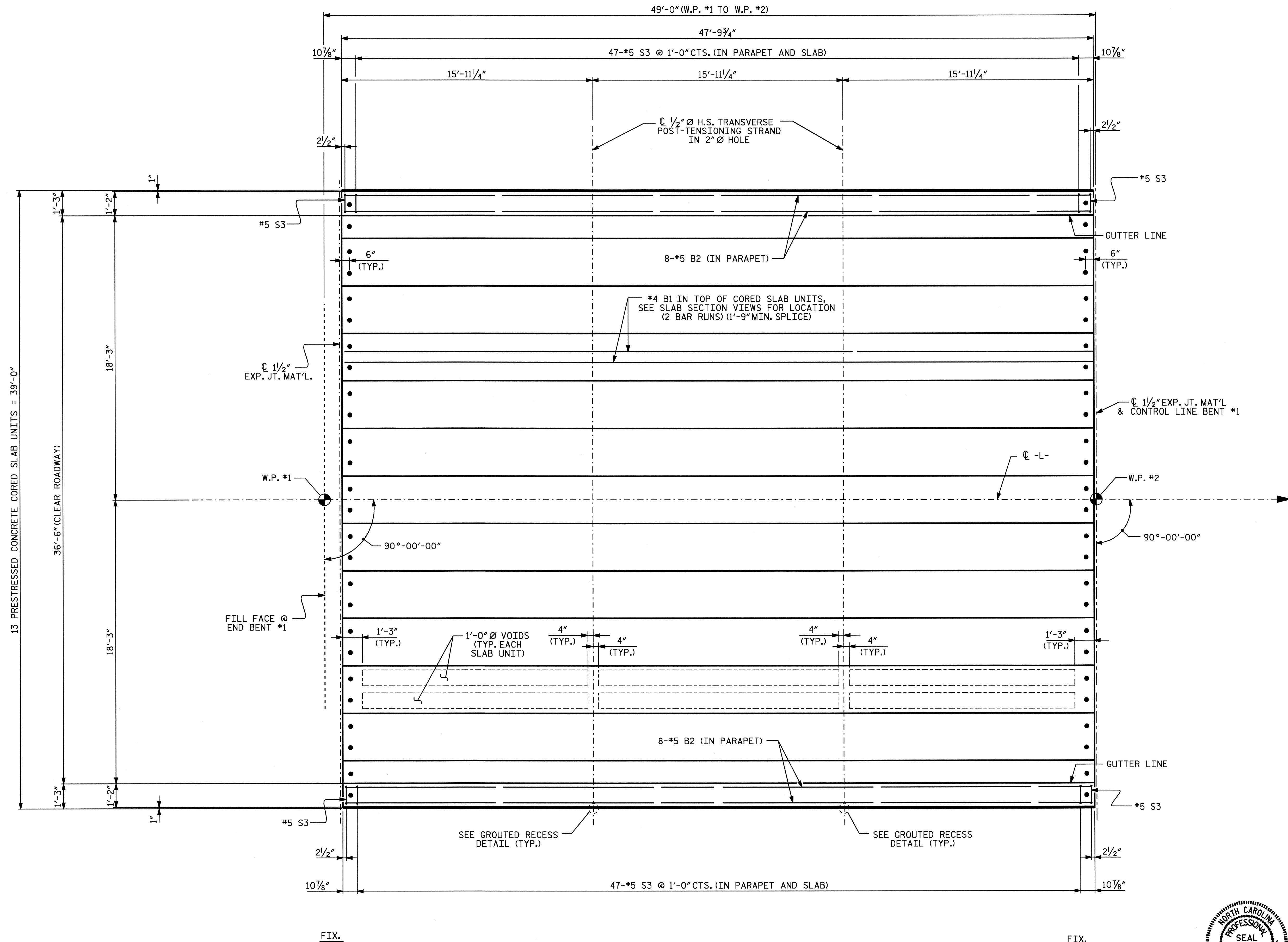
PLAN OF SPAN A
