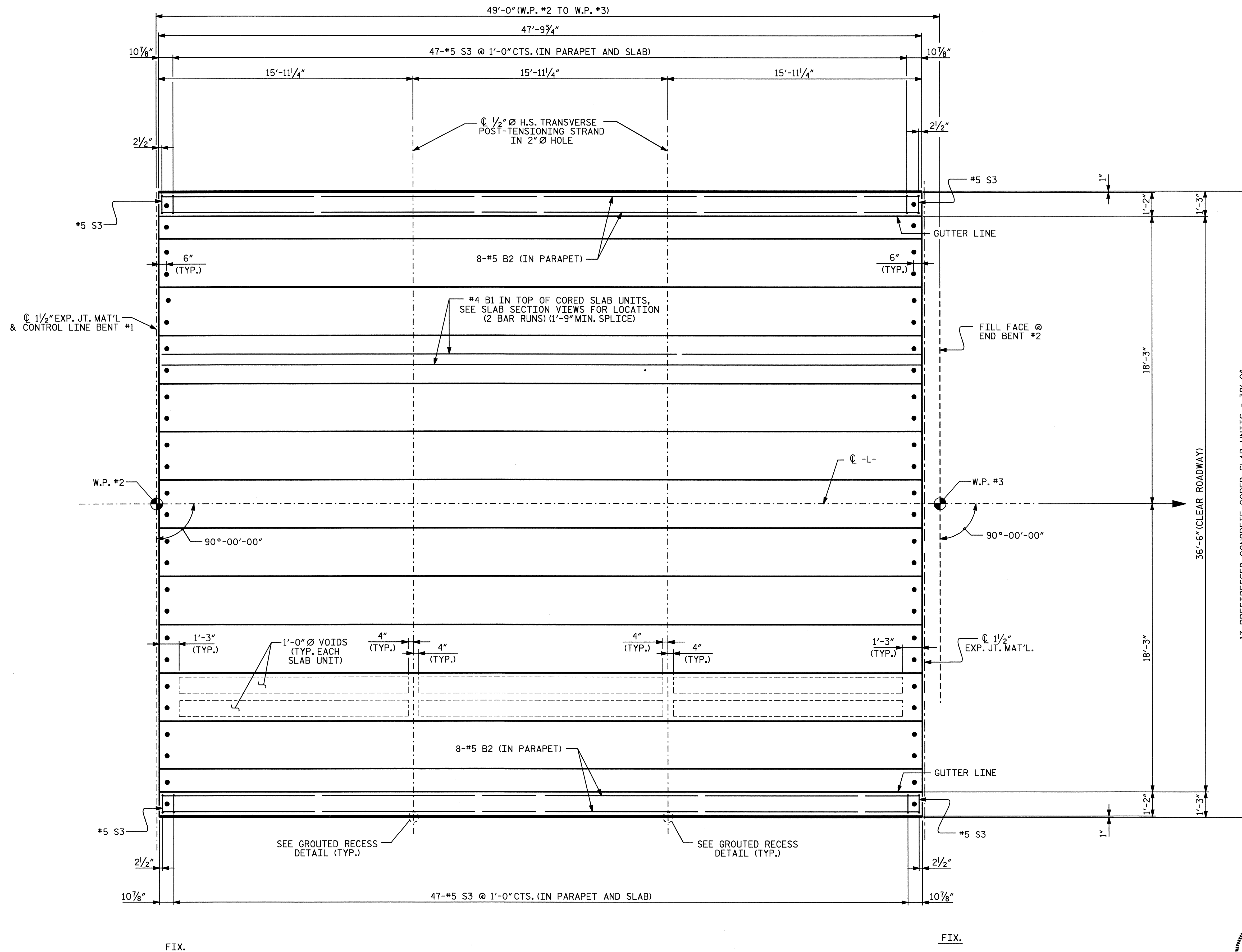
PLAN OF SPAN B
