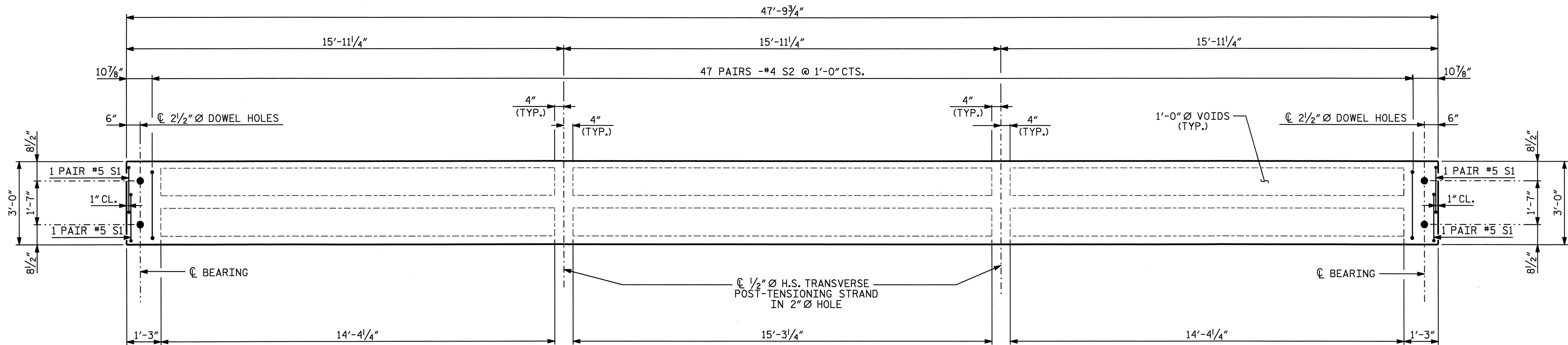
PLAN OF INTERIOR CORED SLAB UNIT (SPAN A & B)
