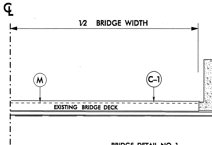
BRIDGE DETAIL NO. 1
