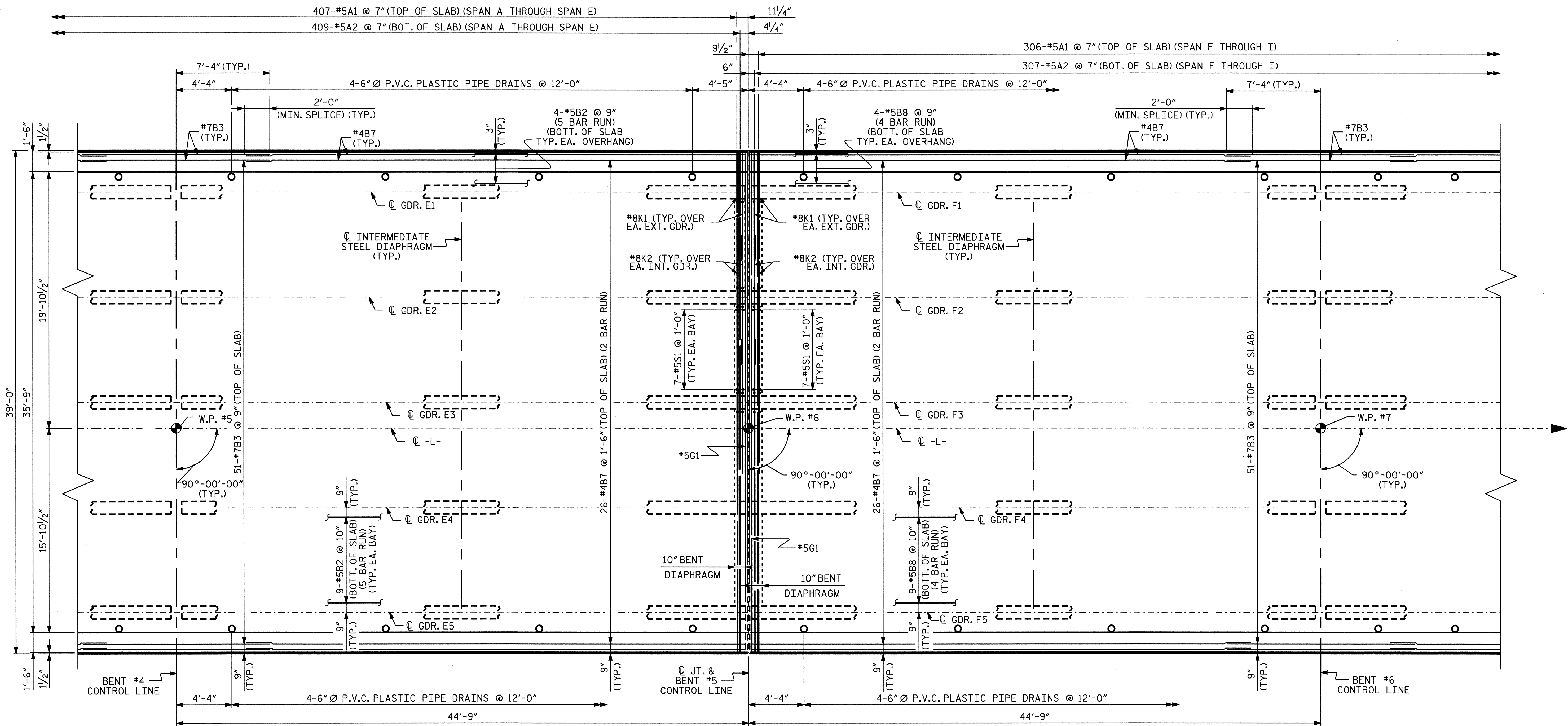
PLAN OF SPAN E
