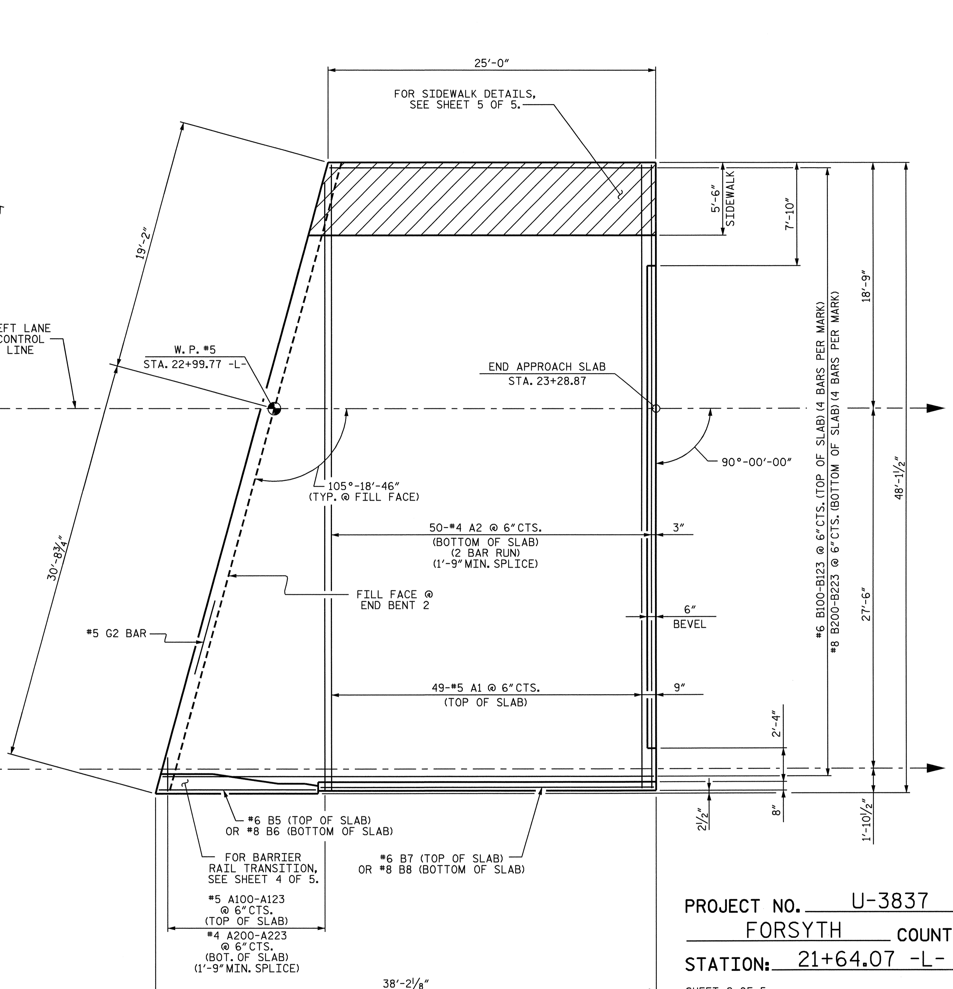
PLAN OF APPROACH SLAB @ END BENT 2
