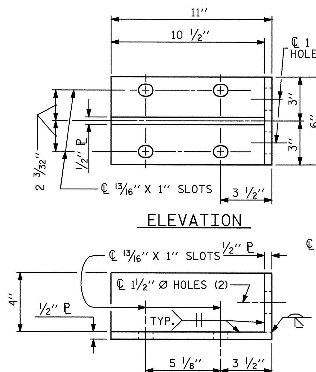
DETAILS FOR ATTACHMENT BRACKET (BOTTOM RAIL ONLY)
