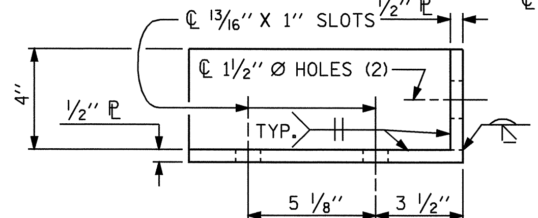
DETAILS FOR ATTACHMENT BRACKET (BOTTOM RAIL ONLY)
