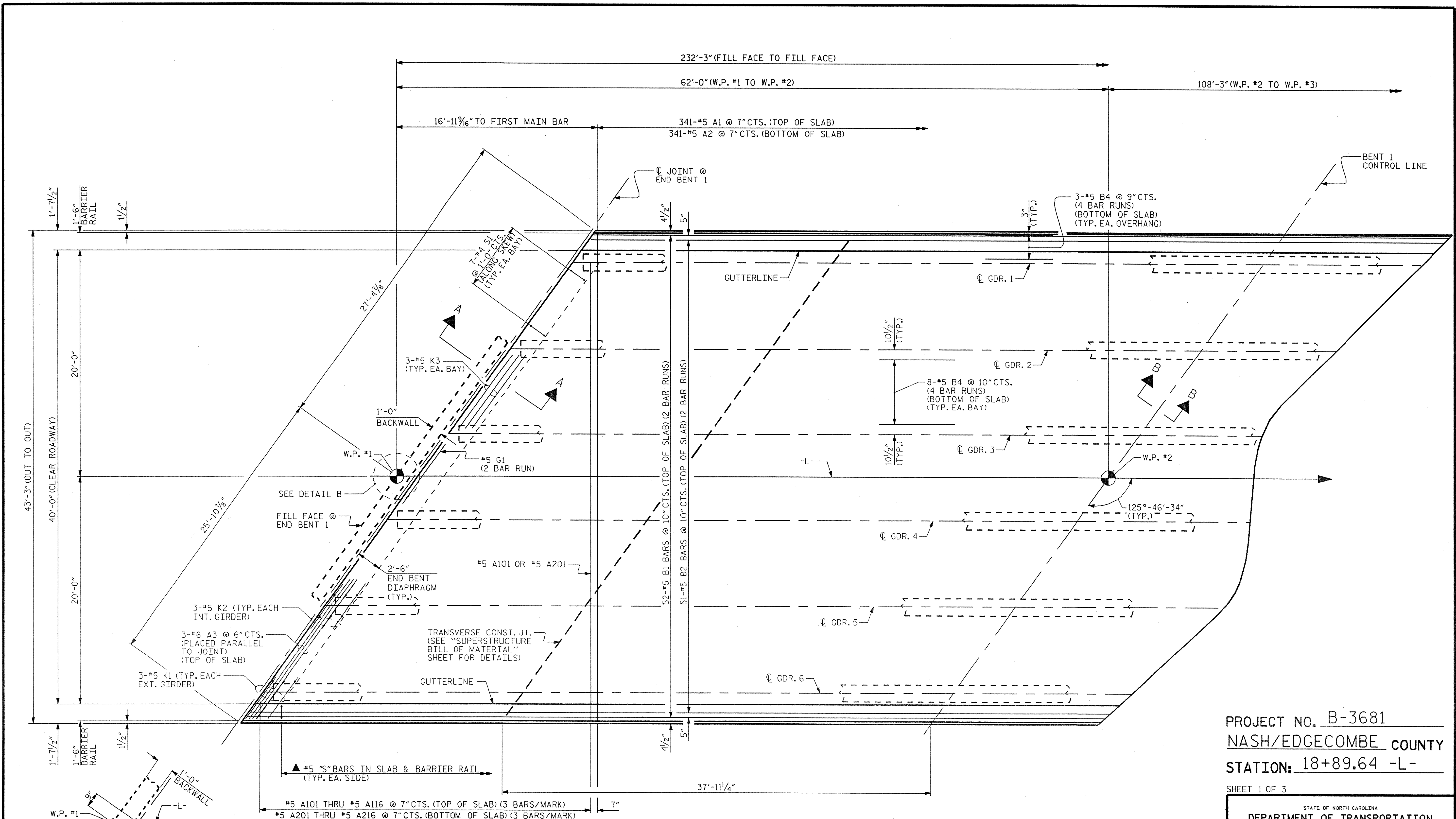
PLAN OF SPAN A
