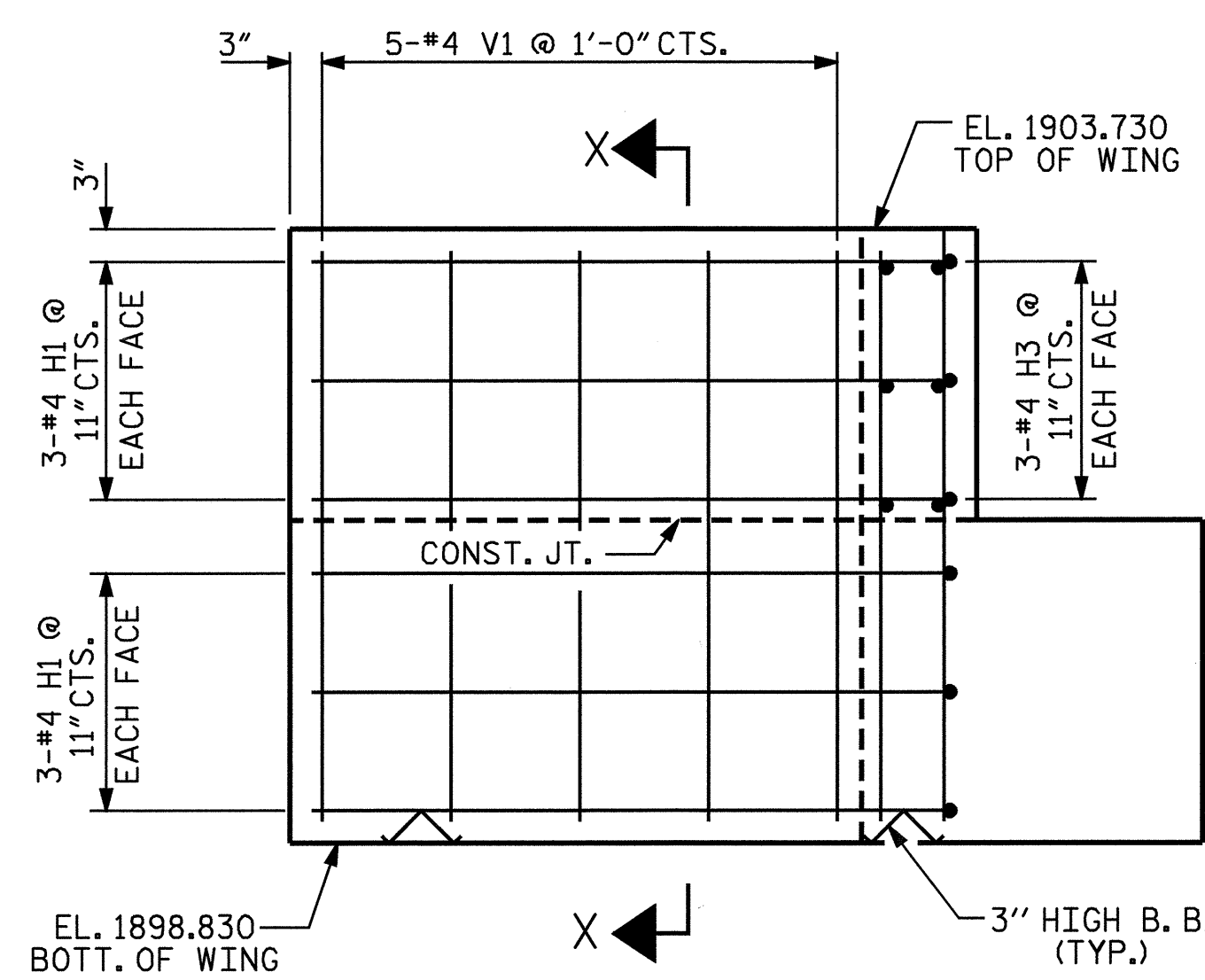
ELEVATION OF WING W1
