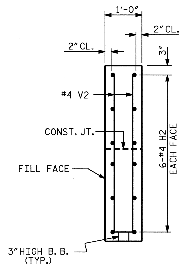
SECTION Y-Y
