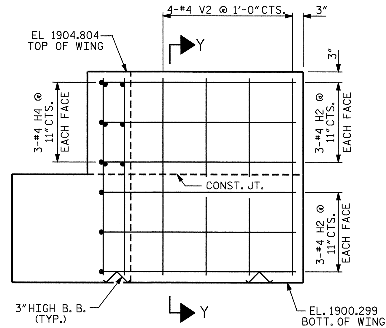
ELEVATION OF WING W2
