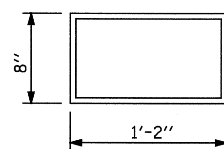
E1 (32 REQ'D) PLAN VIEW OF ELASTOMERIC BEARING TYPE II
