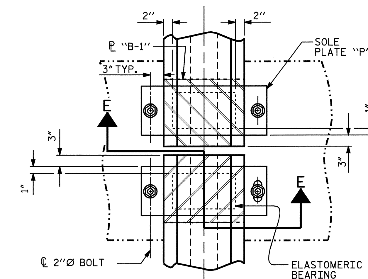
TYPICAL HALF-PLAN
