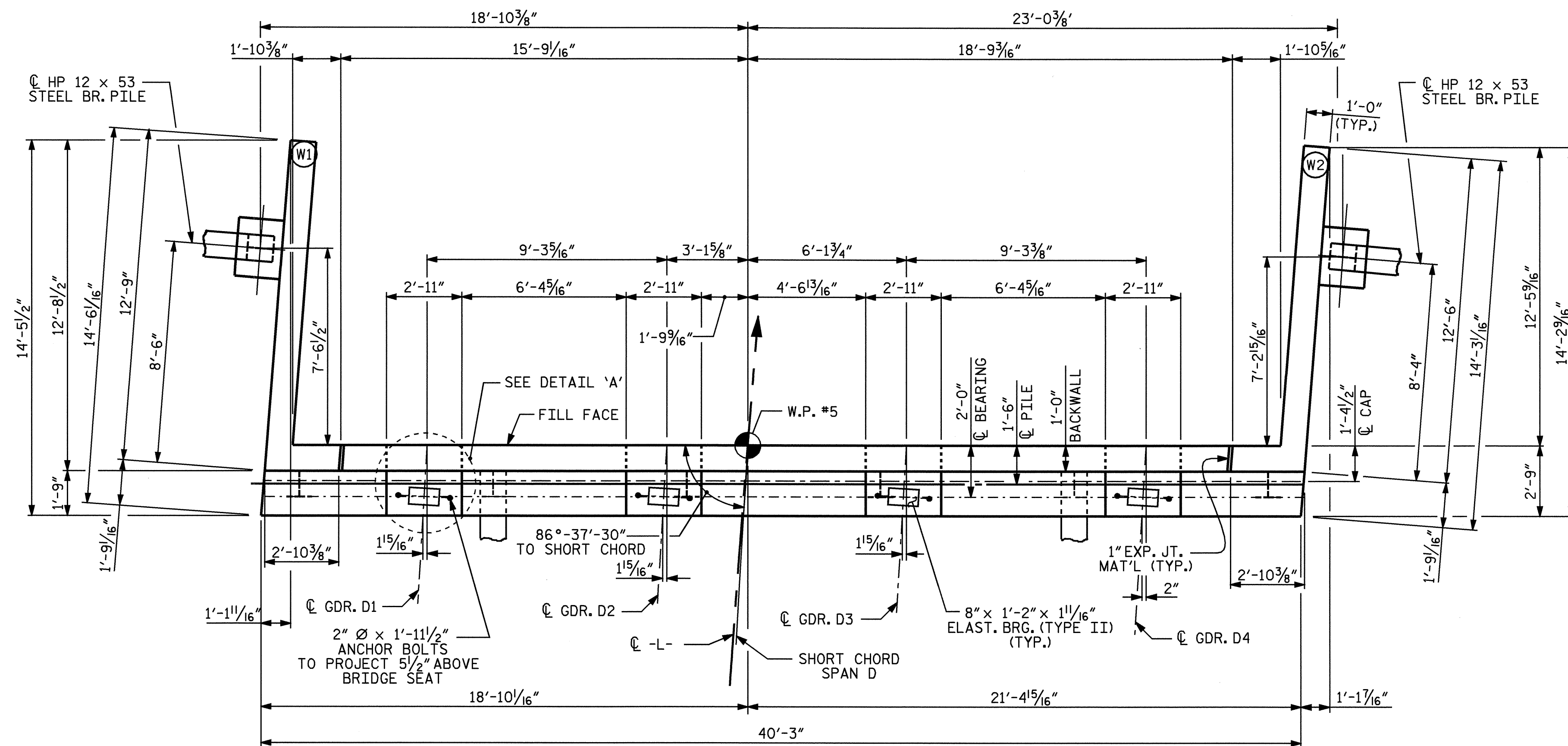
PLAN
