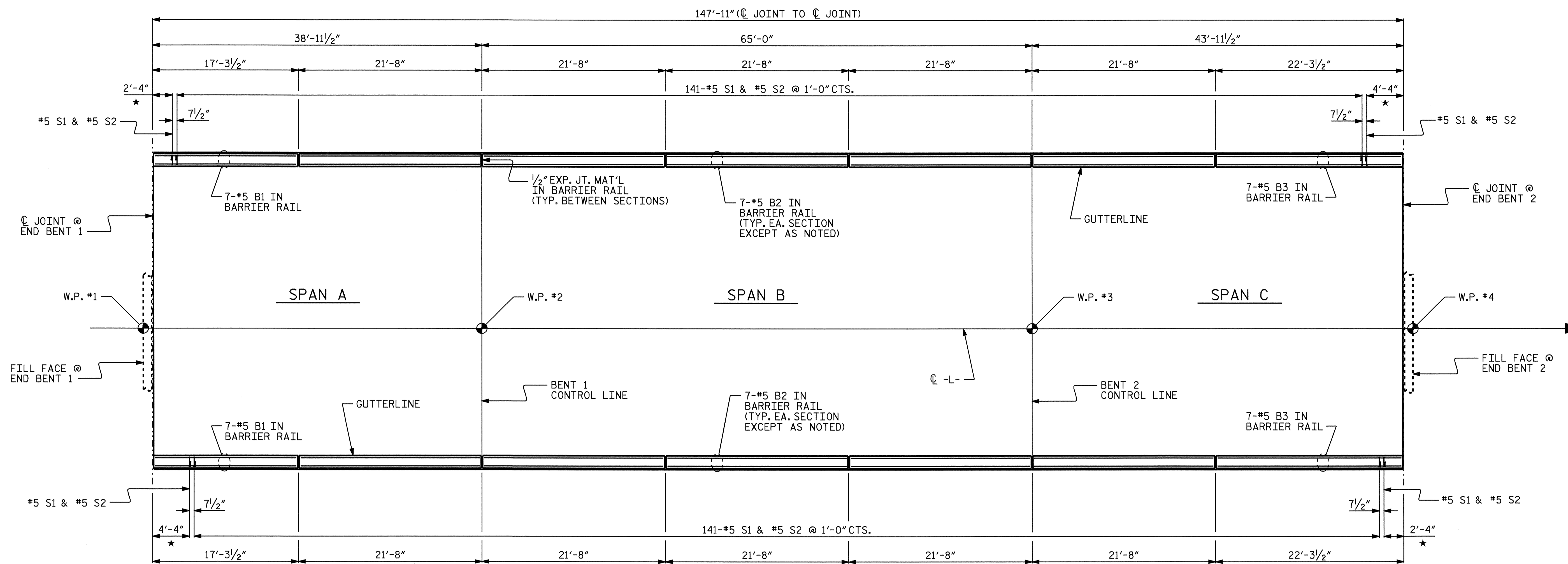
PLAN OF BARRIER RAIL
