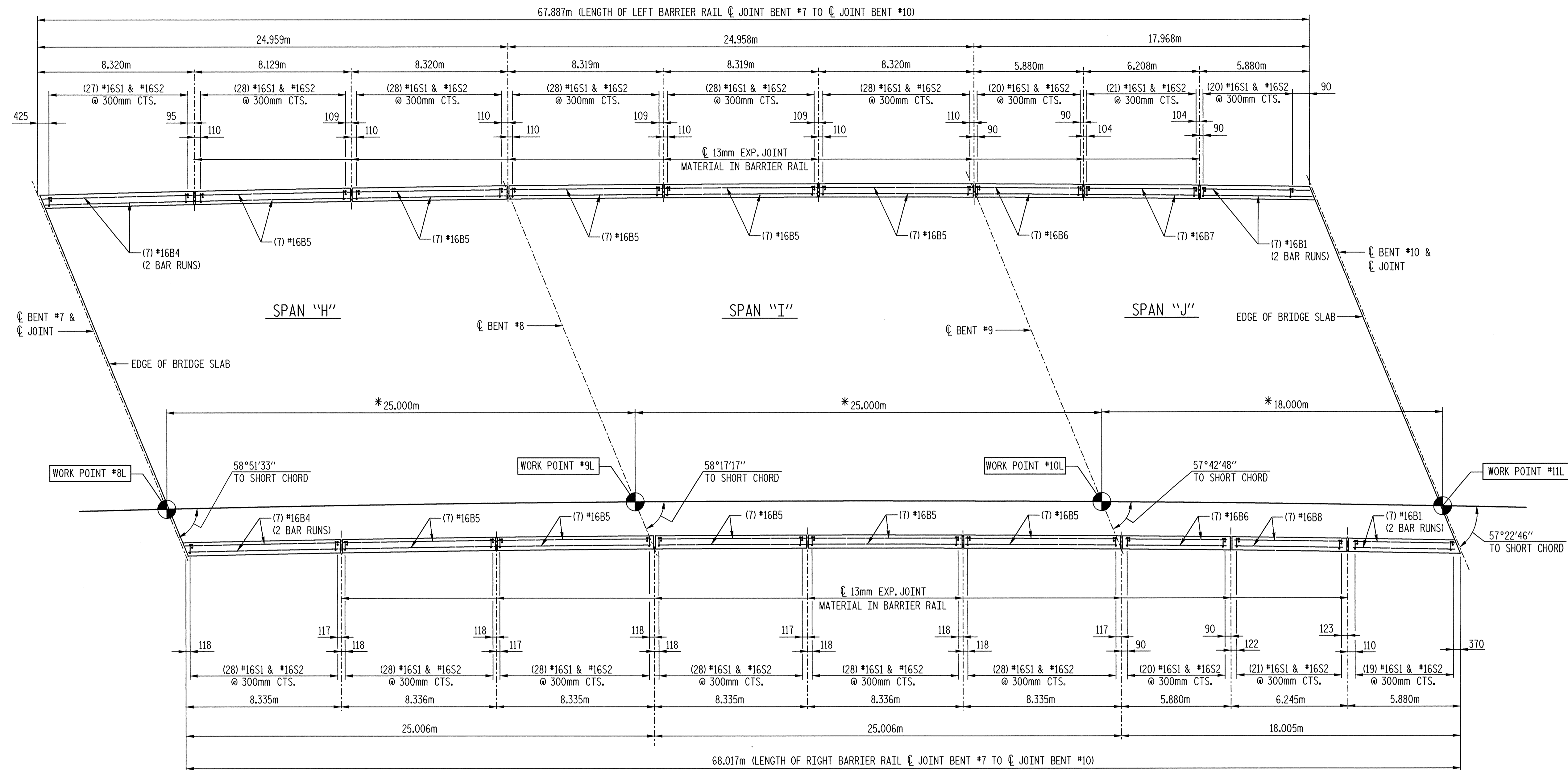
PLAN OF BARRIER RAIL *DIMENSIONS ALONG SHORT CHORD
