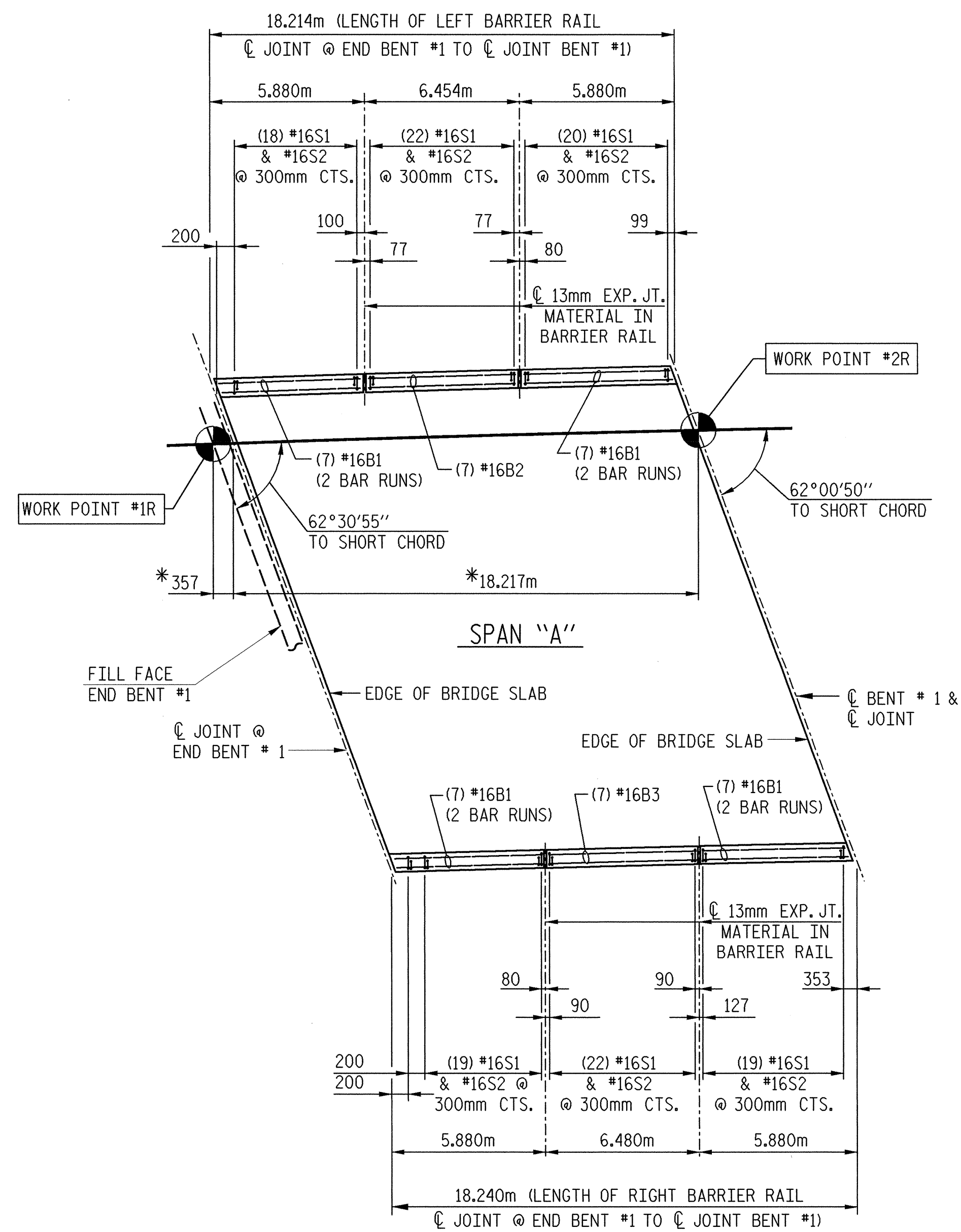
PLAN OF BARRIER RAIL
