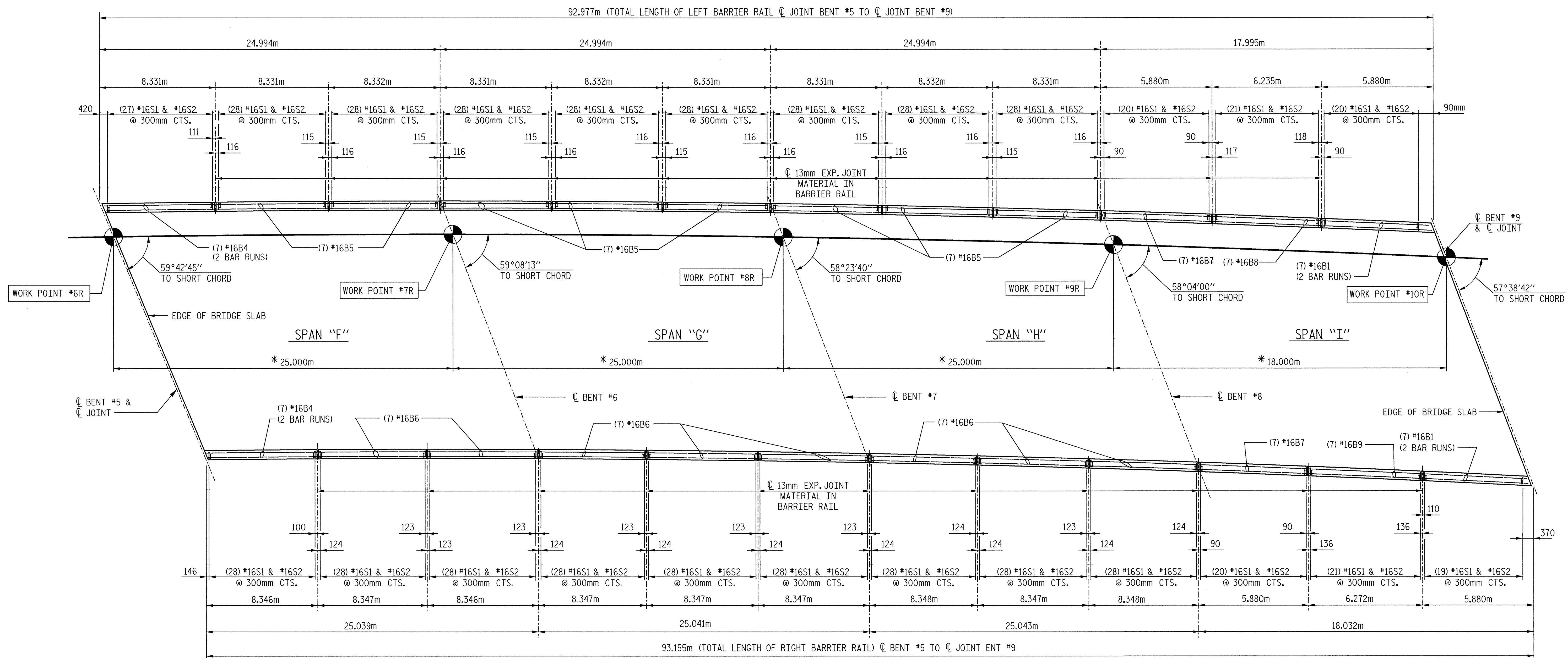
PLAN OF BARRIER RAIL * DIMENSIONS ALONG SHORT CHORD
