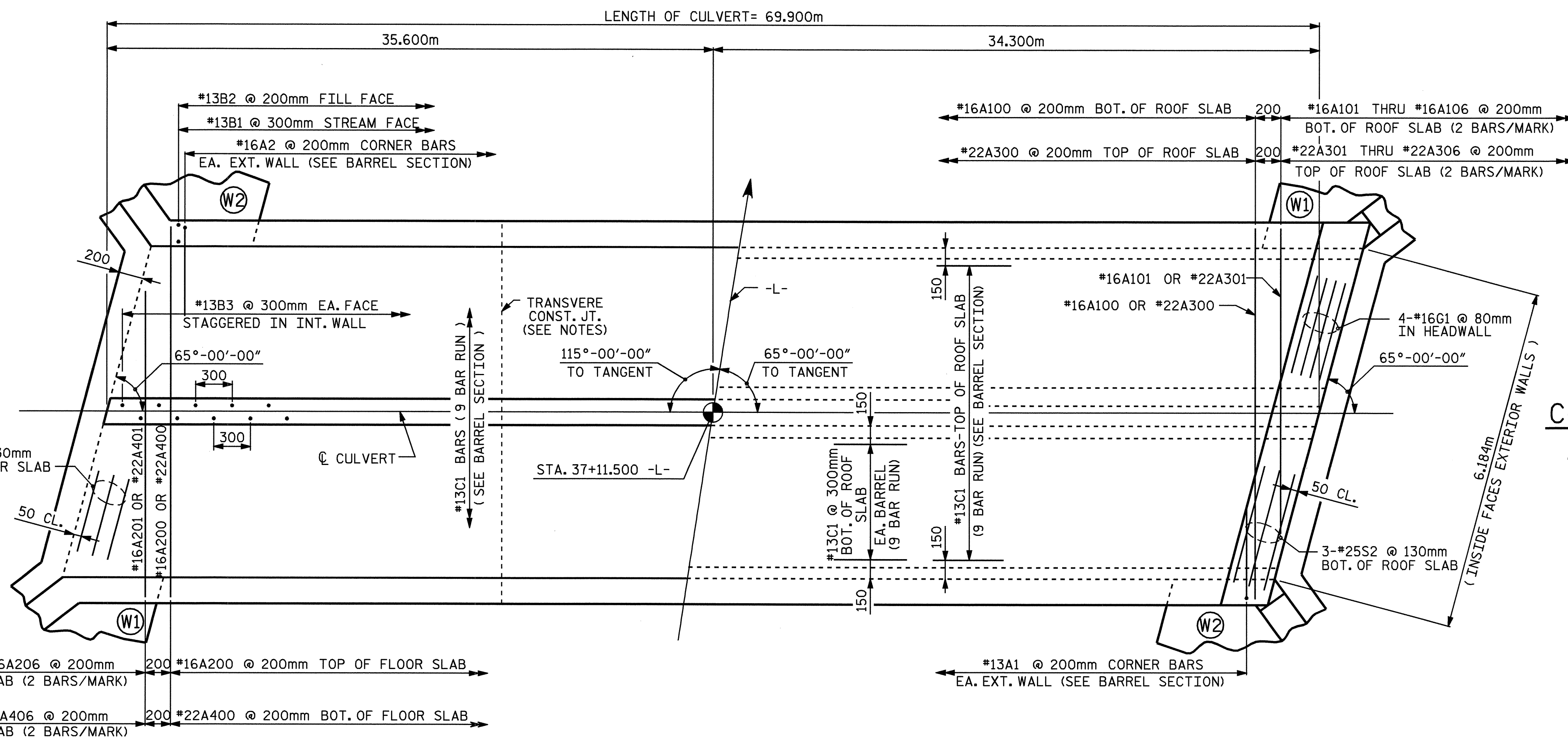
PART PLAN - FLOOR SLAB
