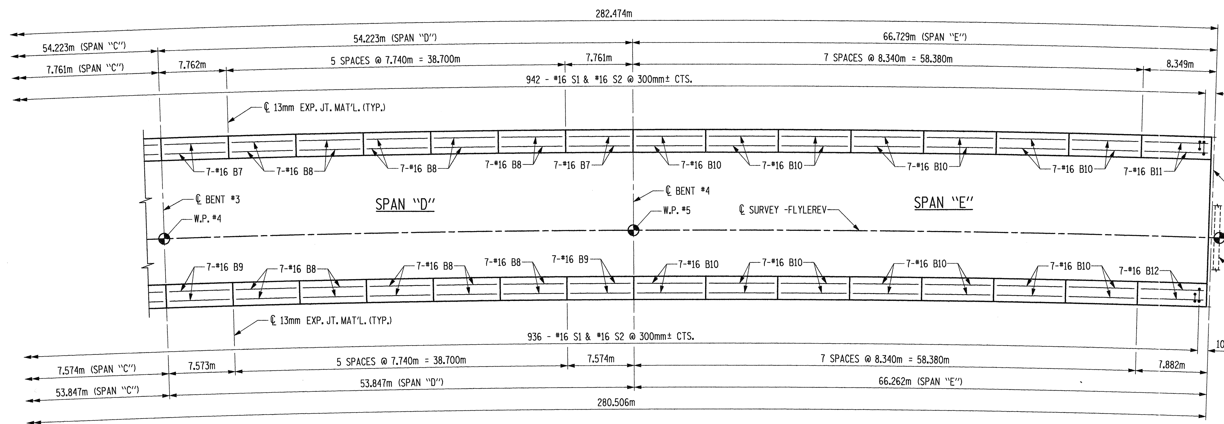
PART PLAN - SPANS "D" AND "E"
