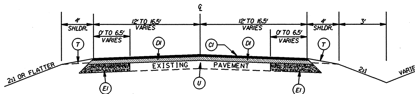
TYPICAL SECTION NO. 14 TURN LANE AT CRISMARK SUBDIVISION -L- 15+16.55 TO 21+37.54
