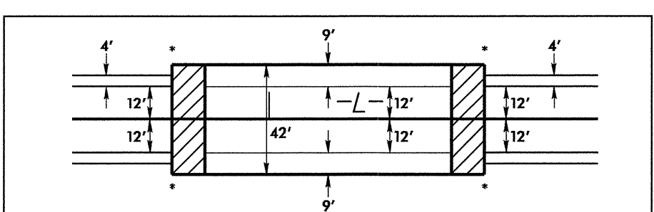
*STRUCTURE ANCHOR UNITS REQUIRED SKETCH SHOWING BRIDGE/PAVEMENT RELATIONSHIP
