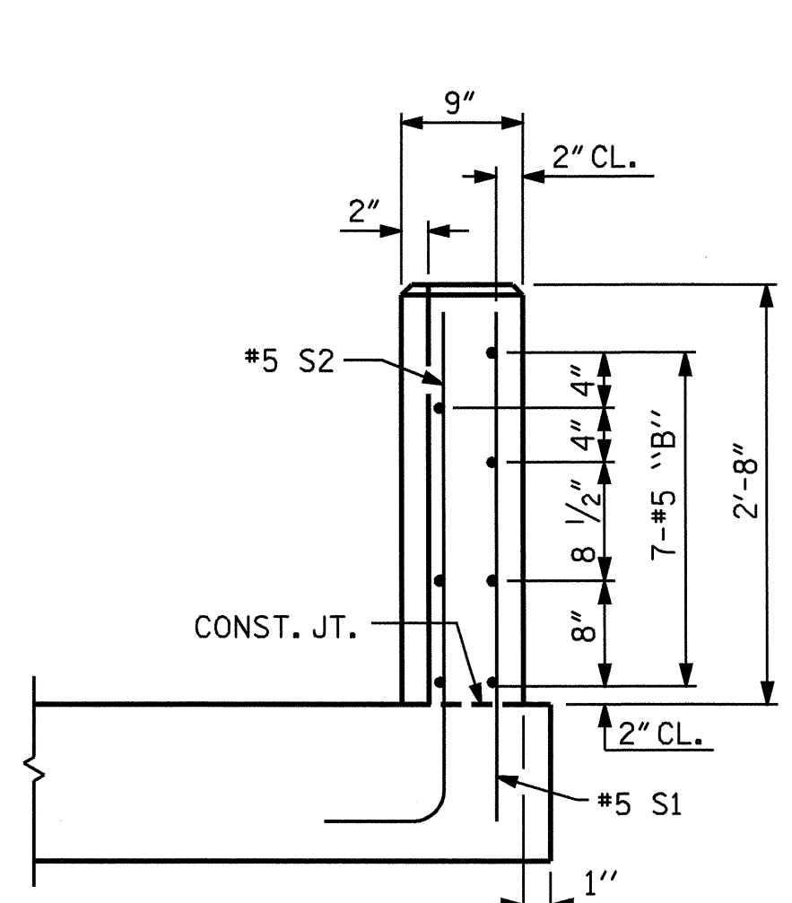
END VIEW
