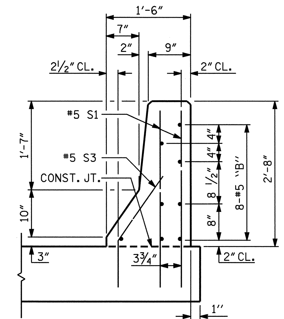
SECTION K-K
