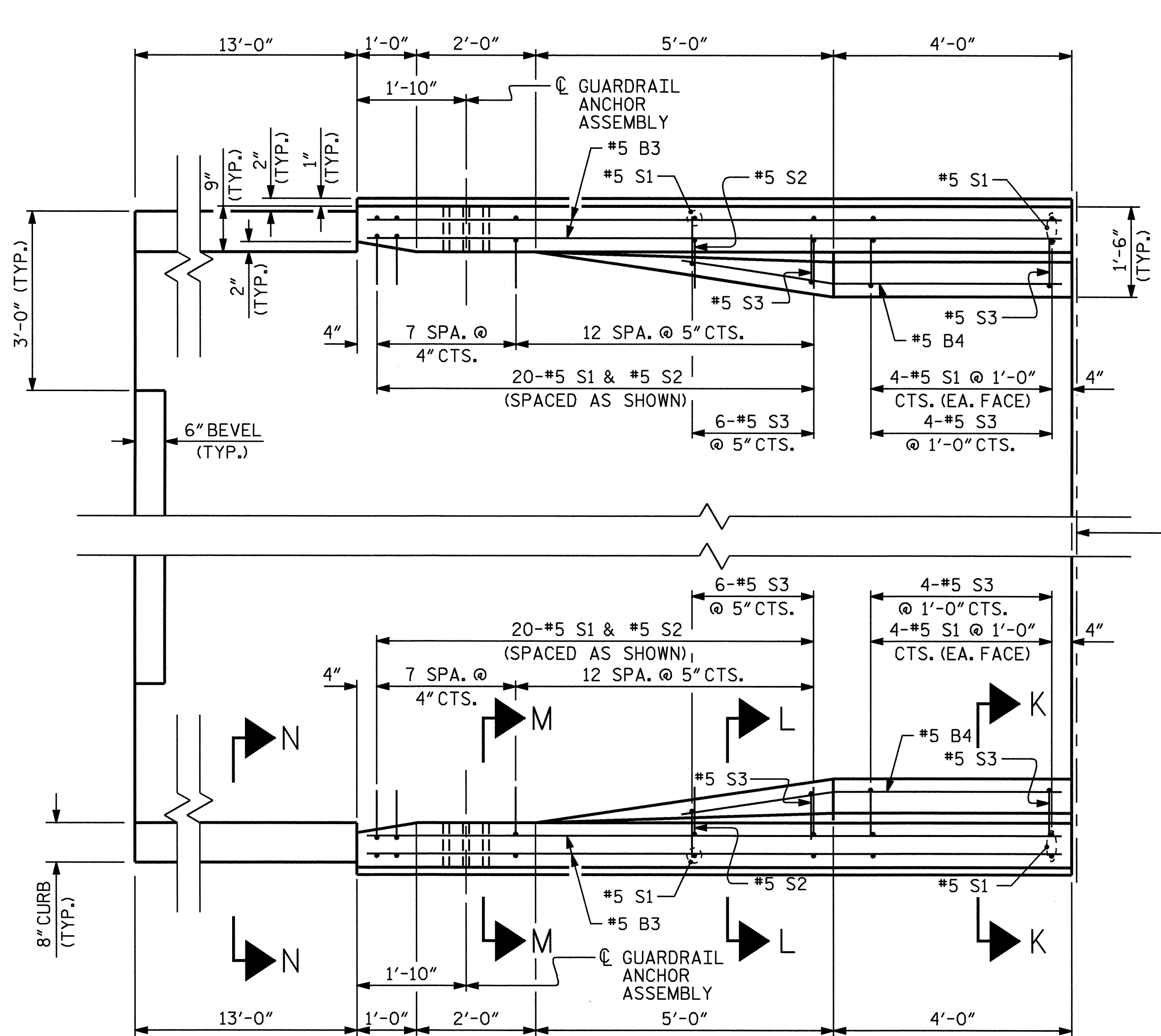
PLAN
