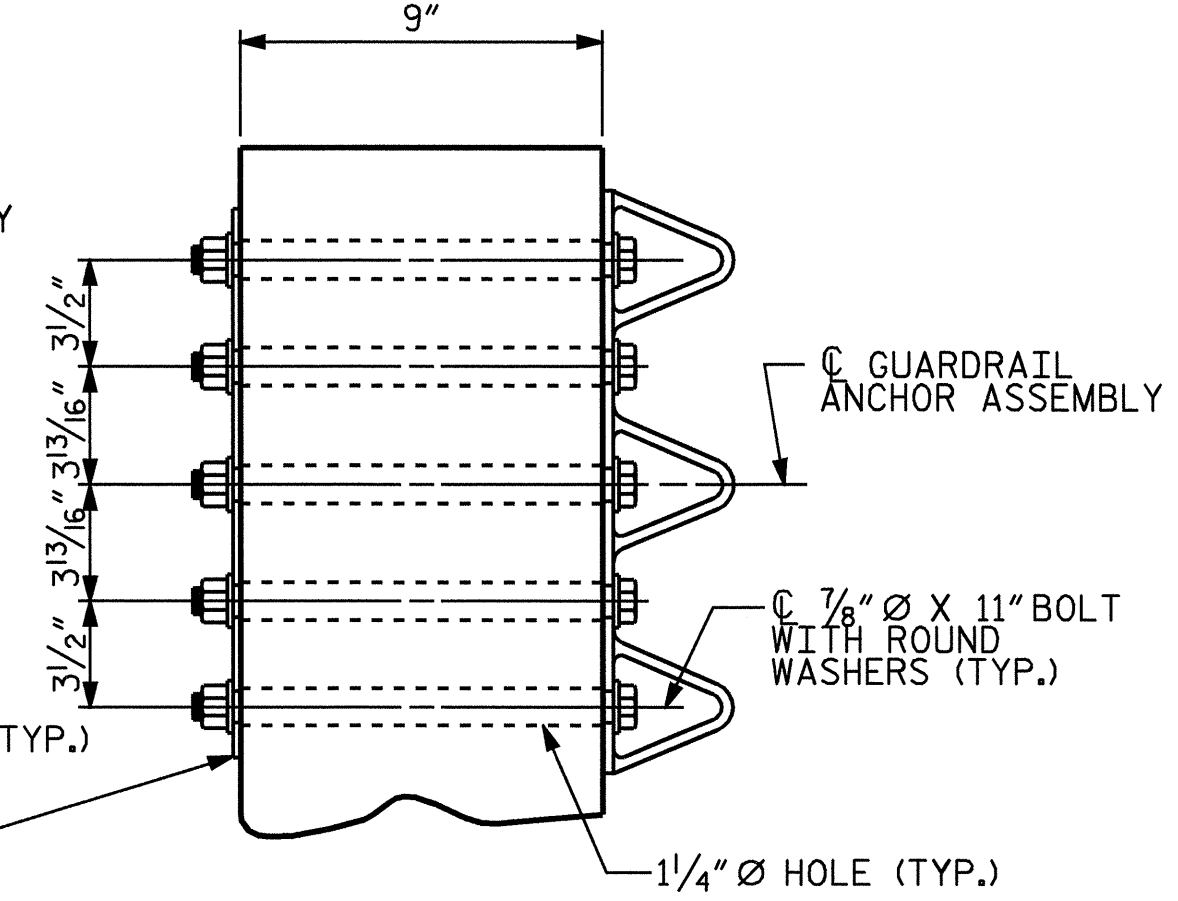
SECTION E-E
