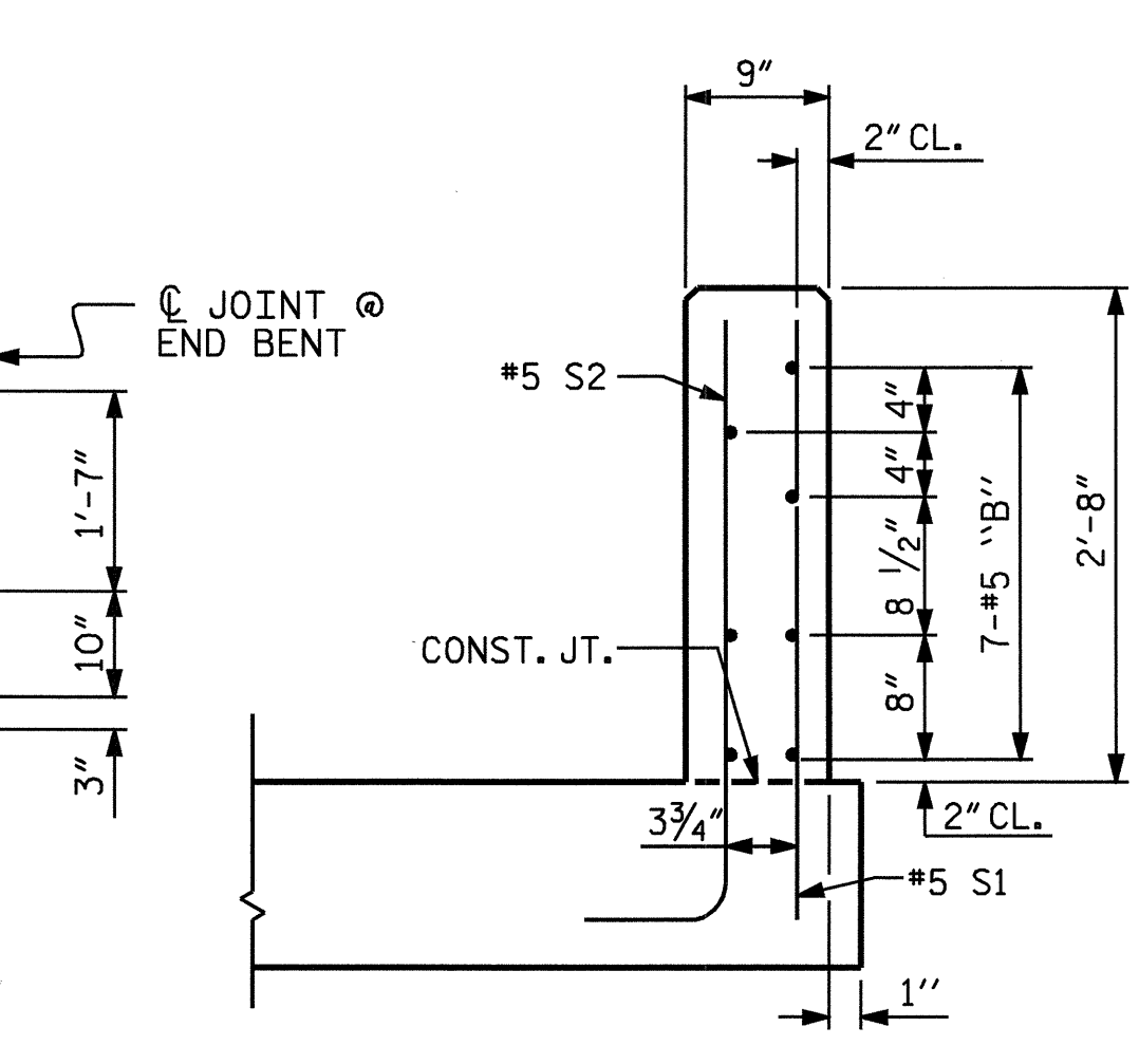
SECTION M-M
