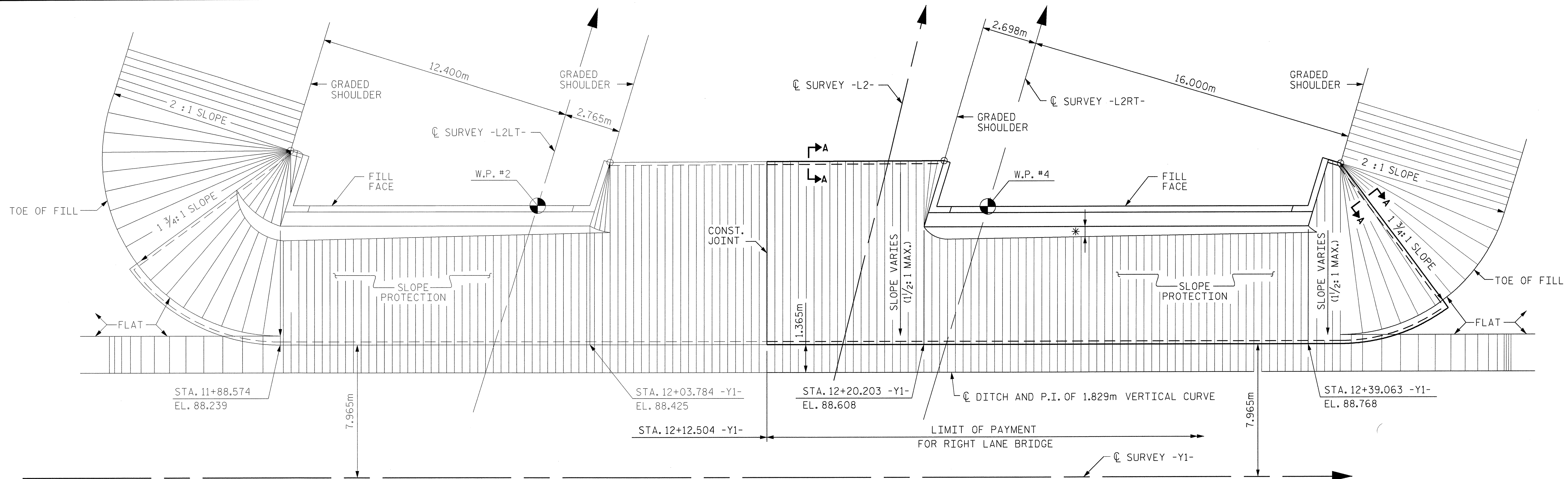
PLAN - END BENT #2 (SLOPE VARIES)
