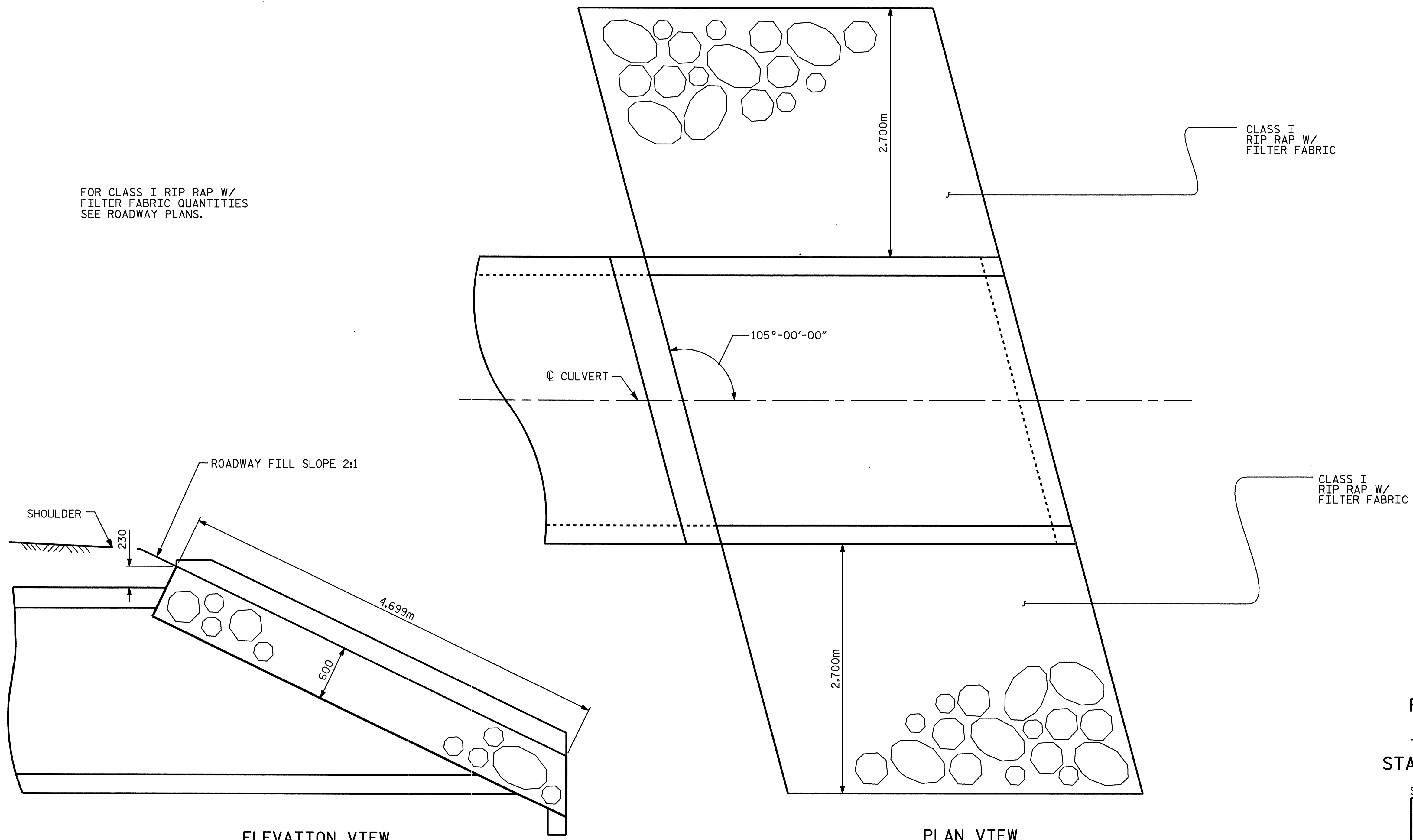
ELEVATION VIEW
