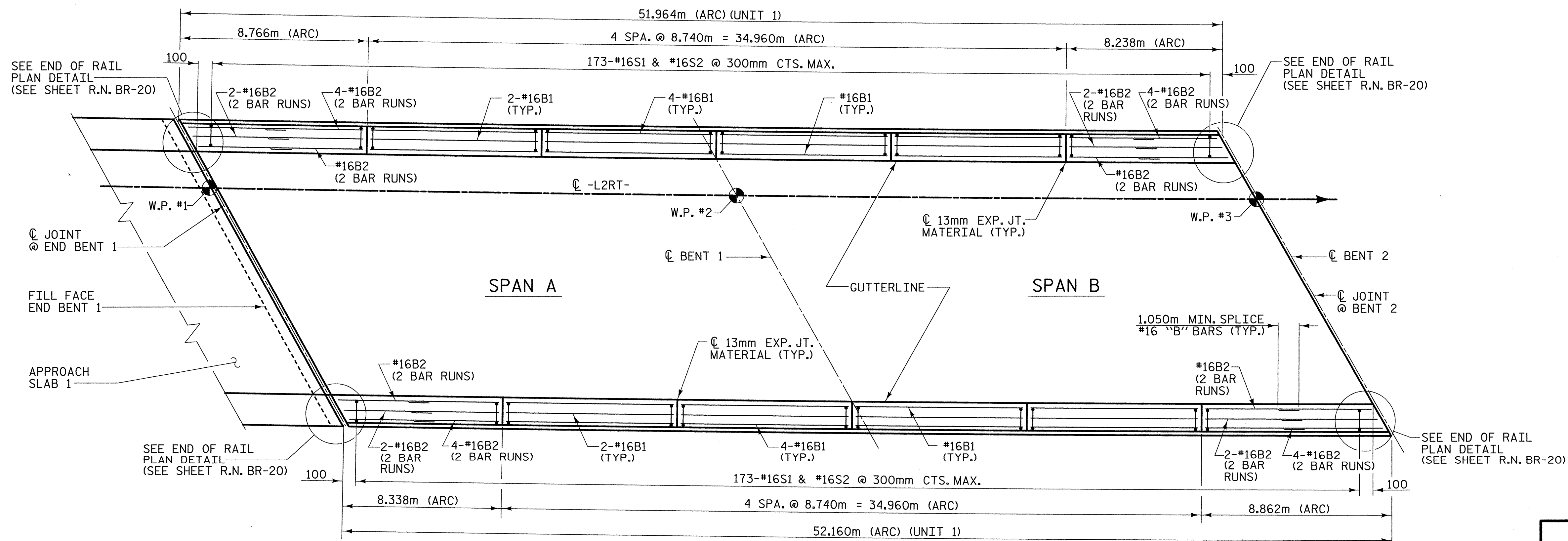
PLAN SPANS A & B
