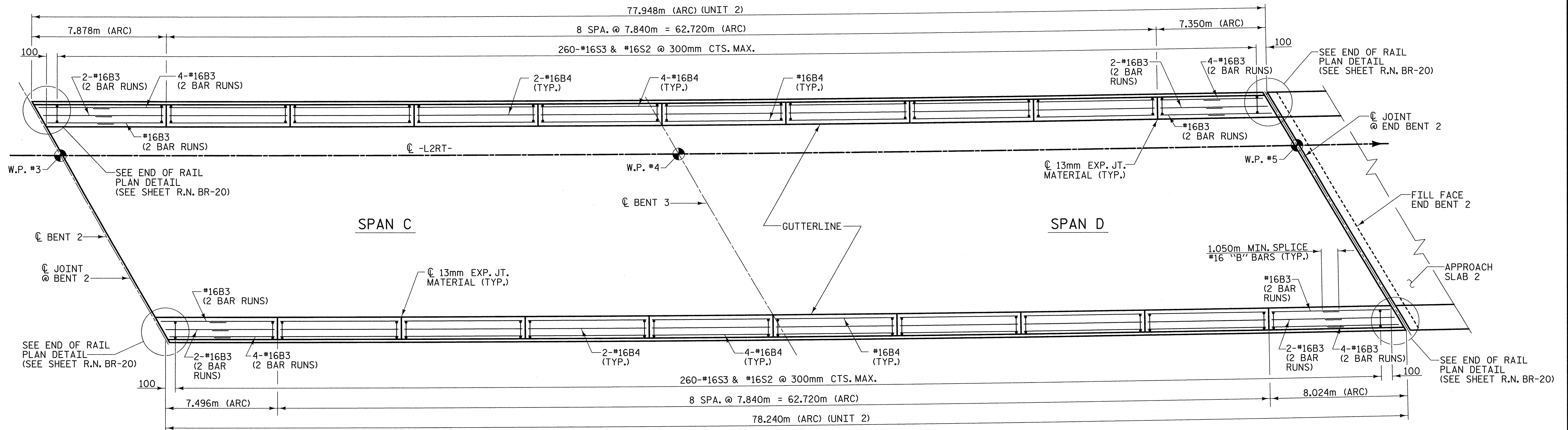
PLAN SPANS C & D
