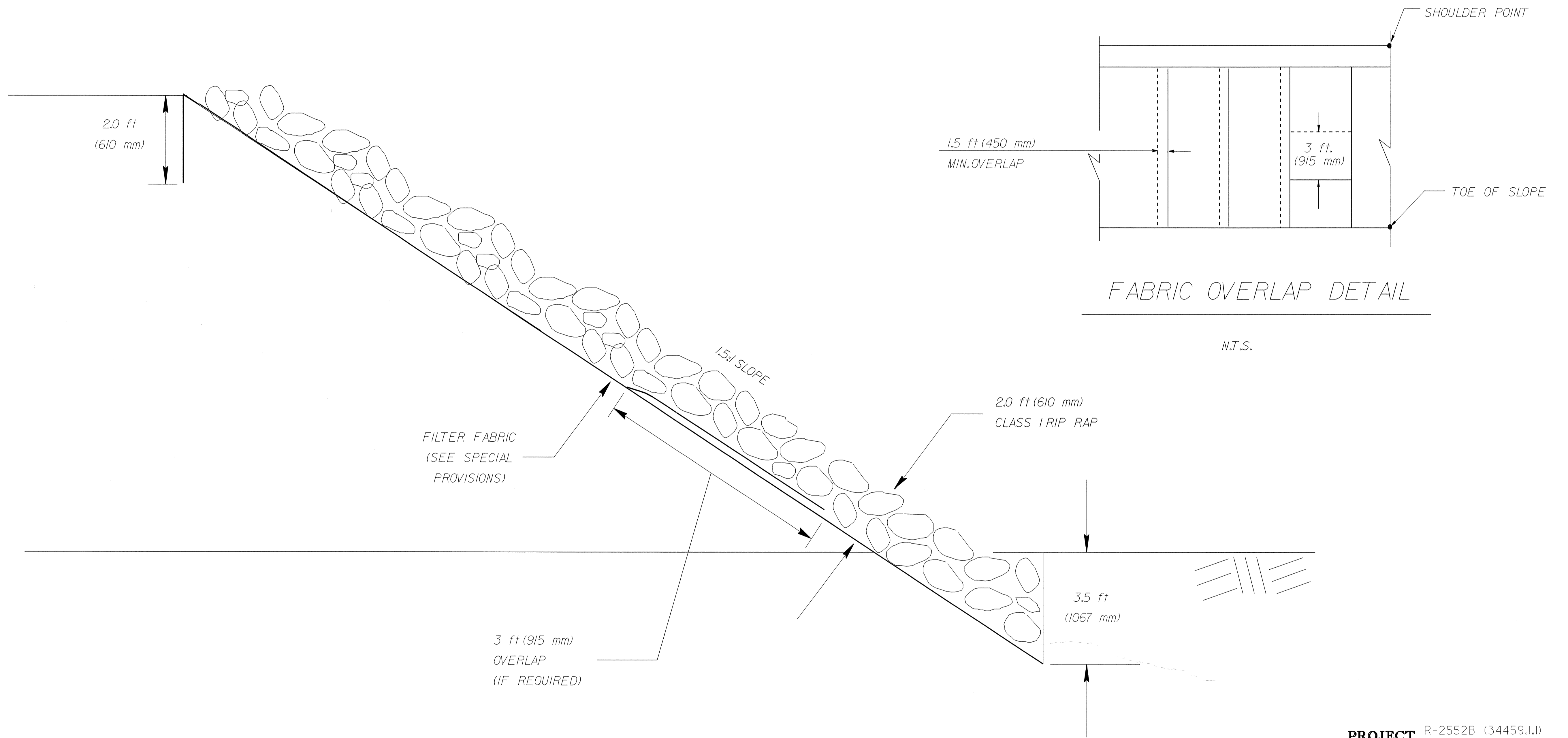
ROCK PLATING DETAIL
