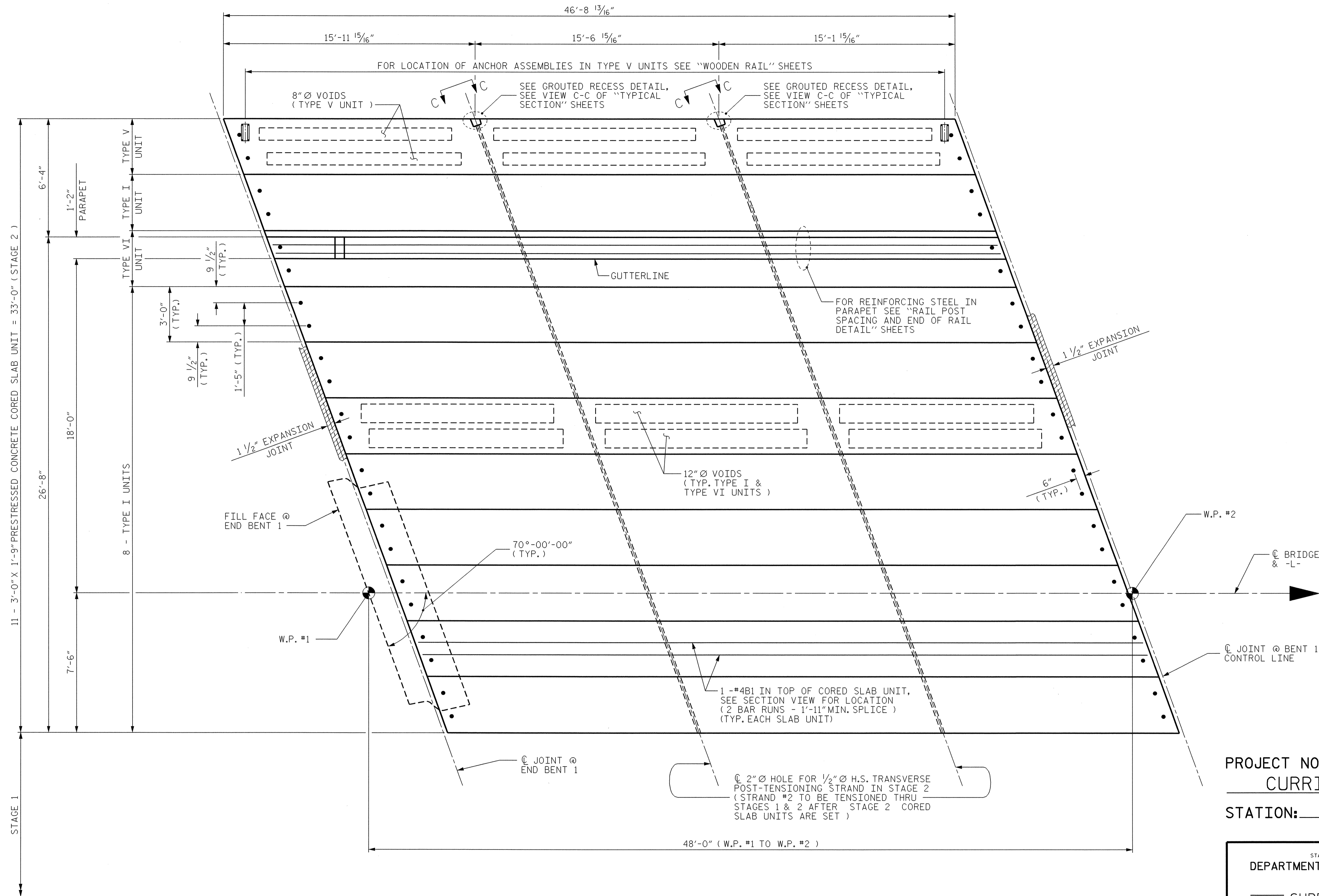
SPAN A FOR PLAN OF TYPE I, V & VI CORED SLAB UNITS, SEE "PLAN OF 3'-0" X 1'-9" CORED SLAB UNIT" FOR DETAILS.
