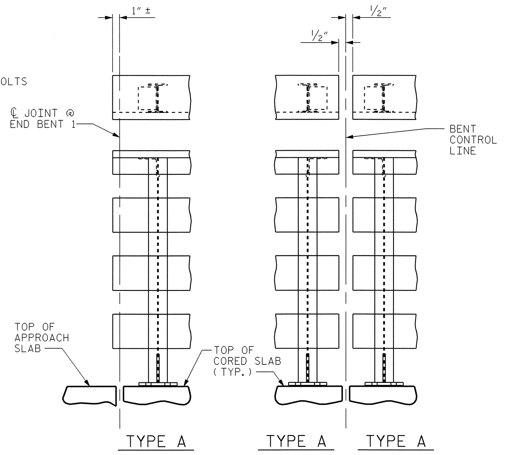
ELEVATION @ END BENTS & BENTS ELEVATION @ END BENT 1 SHOWN. ELEVATION @ END BENT 2 SIMILAR
