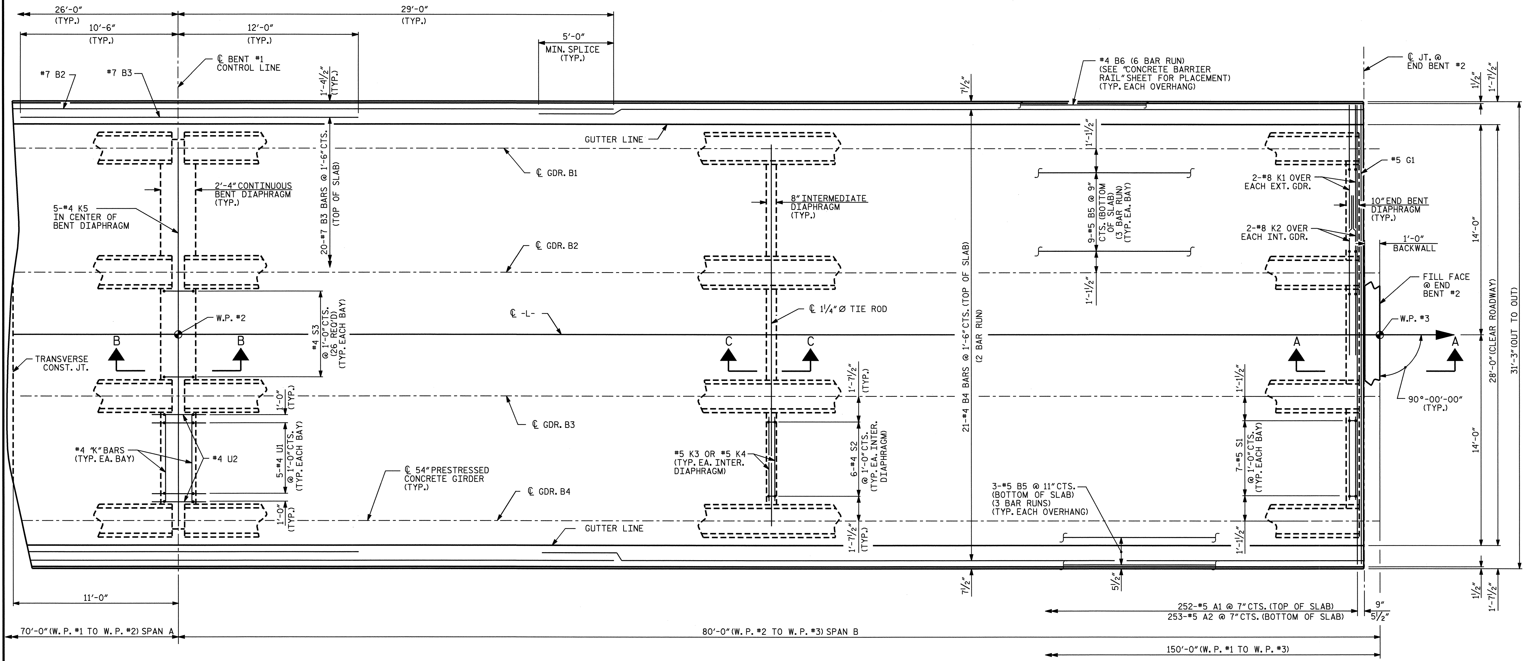
PLAN OF SPAN B (FOR SECTION A-A, B-B AND C-C, SEE "TYPICAL SECTION DETAILS" SHEET 2 OF 2.)
