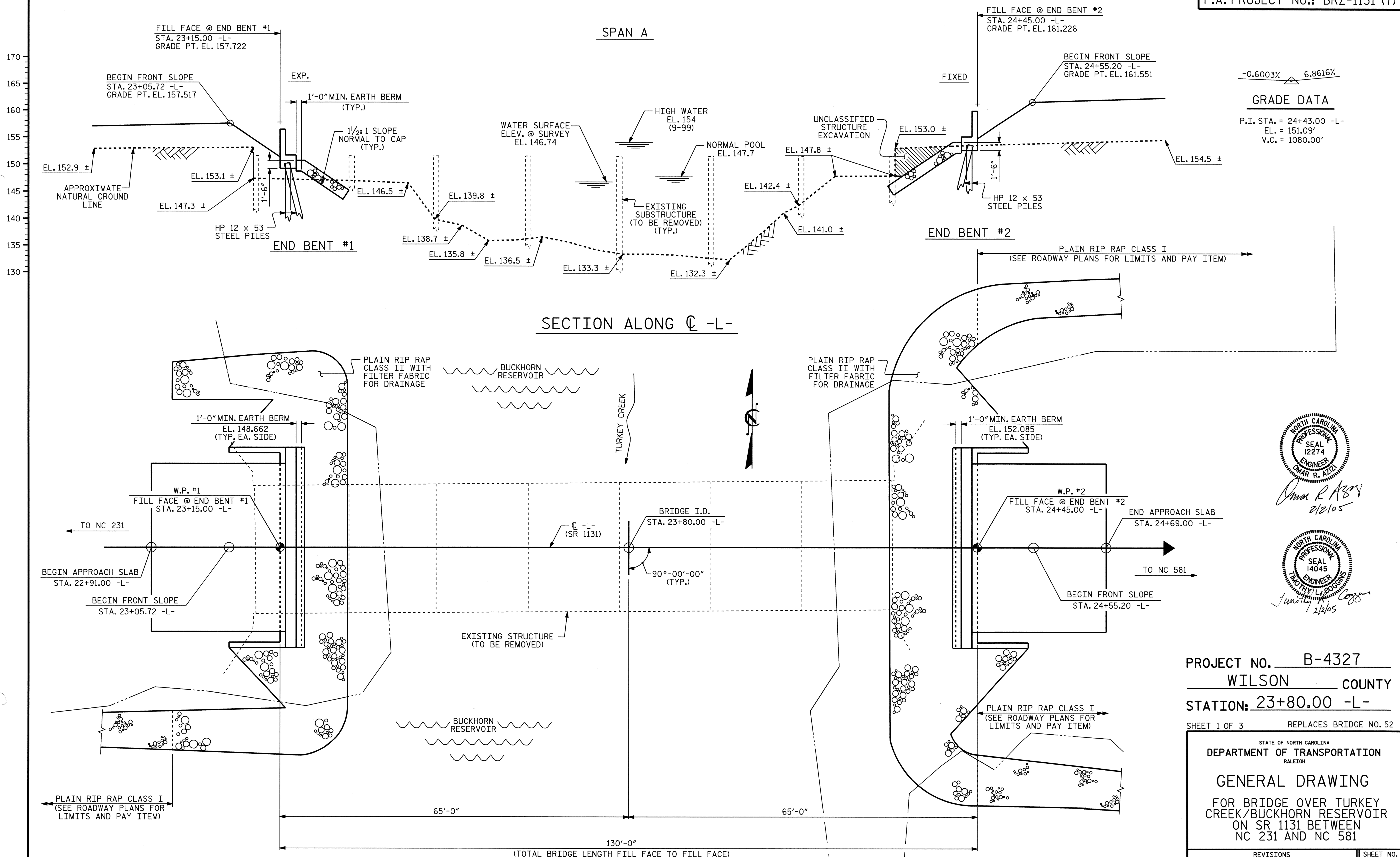
PLAN (PILES NOT SHOWN FOR CLARITY)
