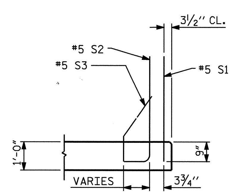
SECTION L-L
