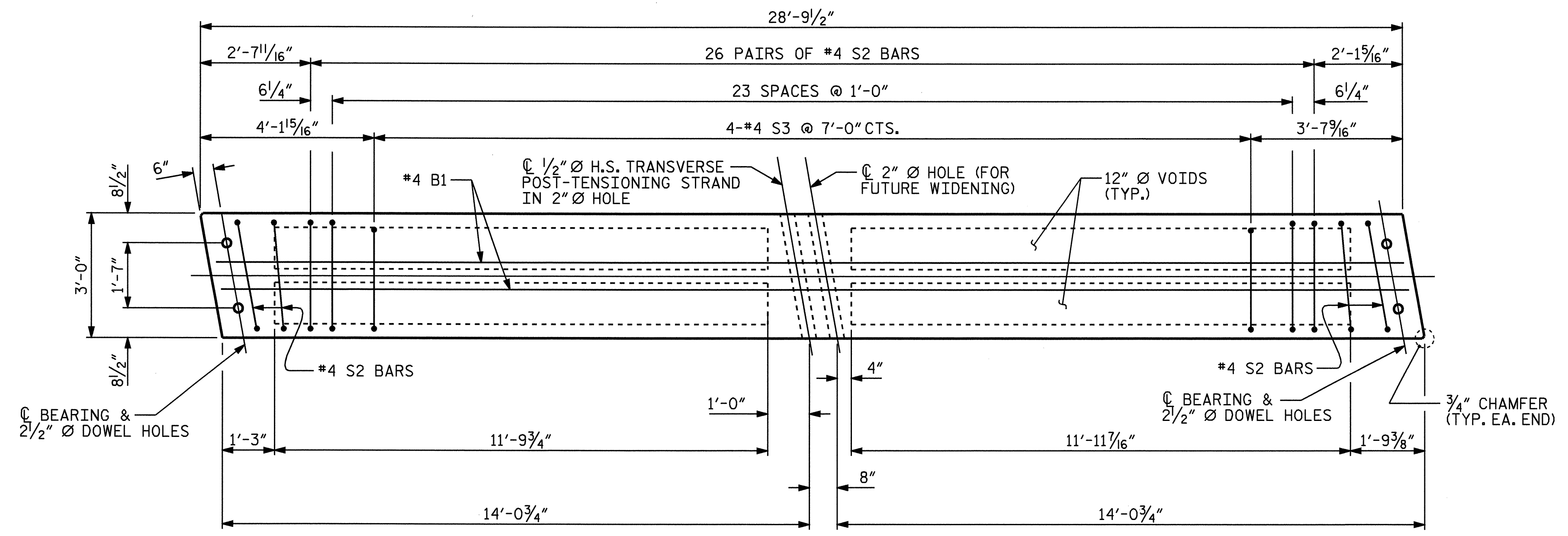
PLAN OF EXTERIOR AND INTERIOR (SIDEWALK) CORED SLAB UNIT - SPAN A AND C
