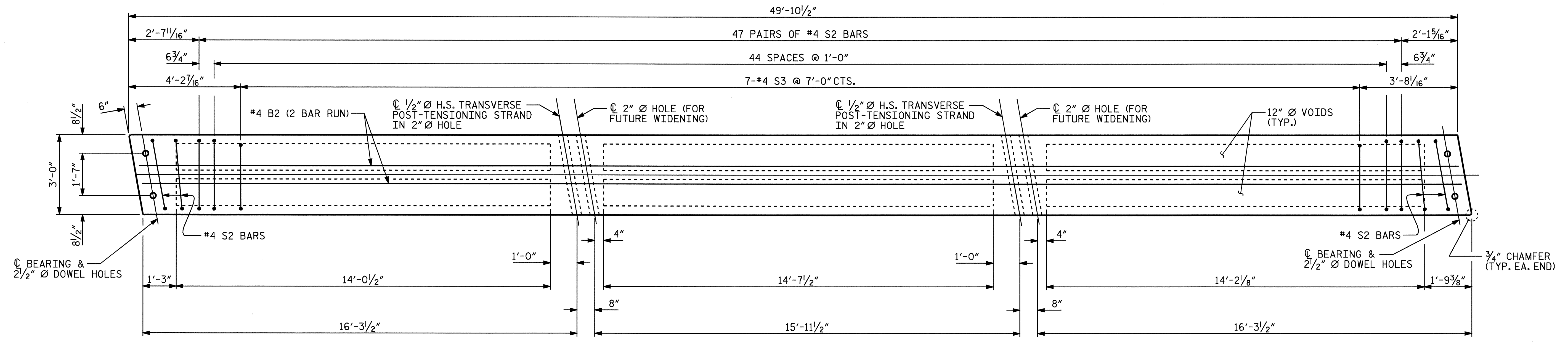
PLAN OF EXTERIOR AND INTERIOR (SIDEWALK) CORED SLAB UNIT - SPAN B
