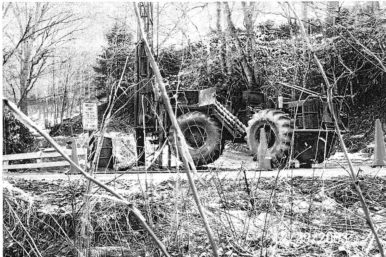
Photograph 1: View of End Bent-1 from Left to Right
