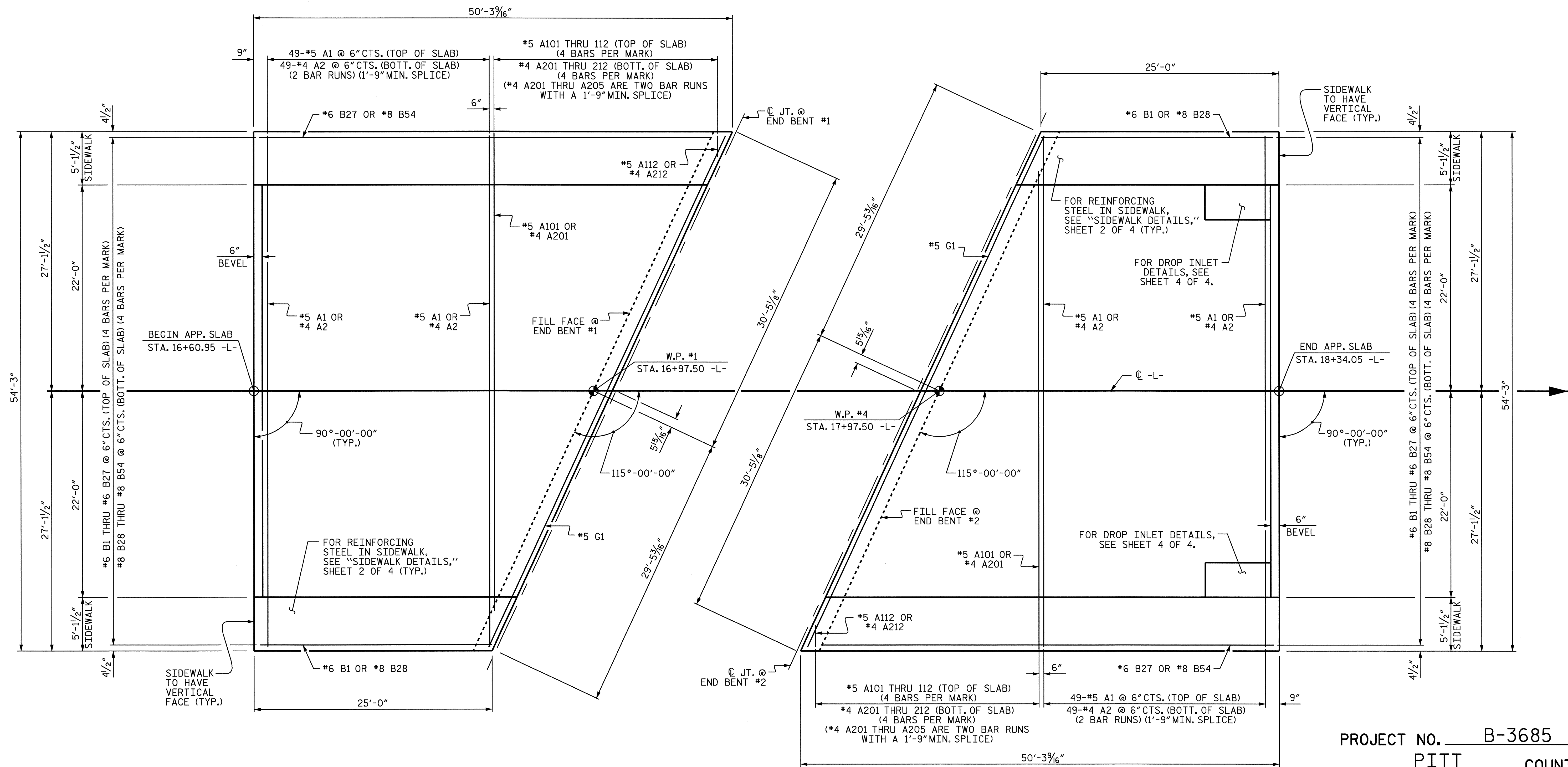
APPROACH SLAB @ END BENT #1
