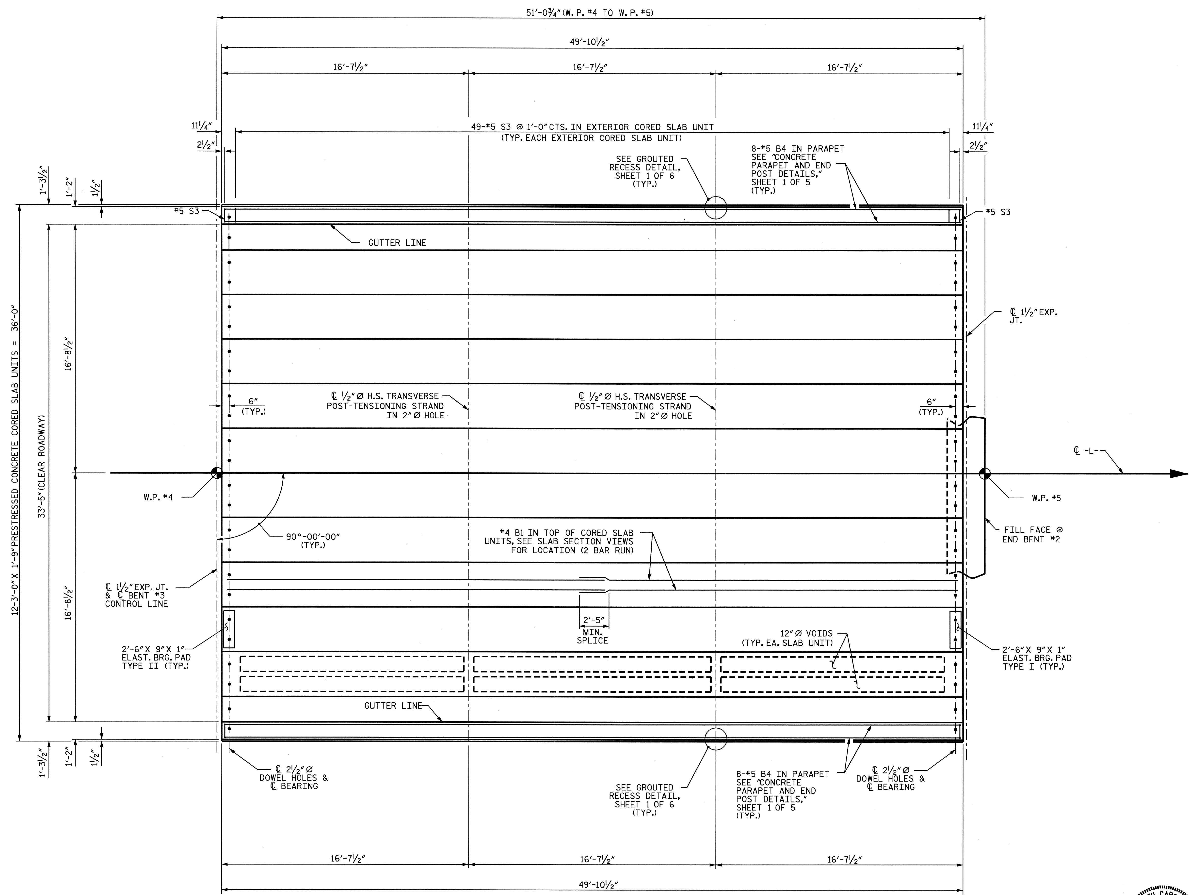
PLAN OF SPAN D
