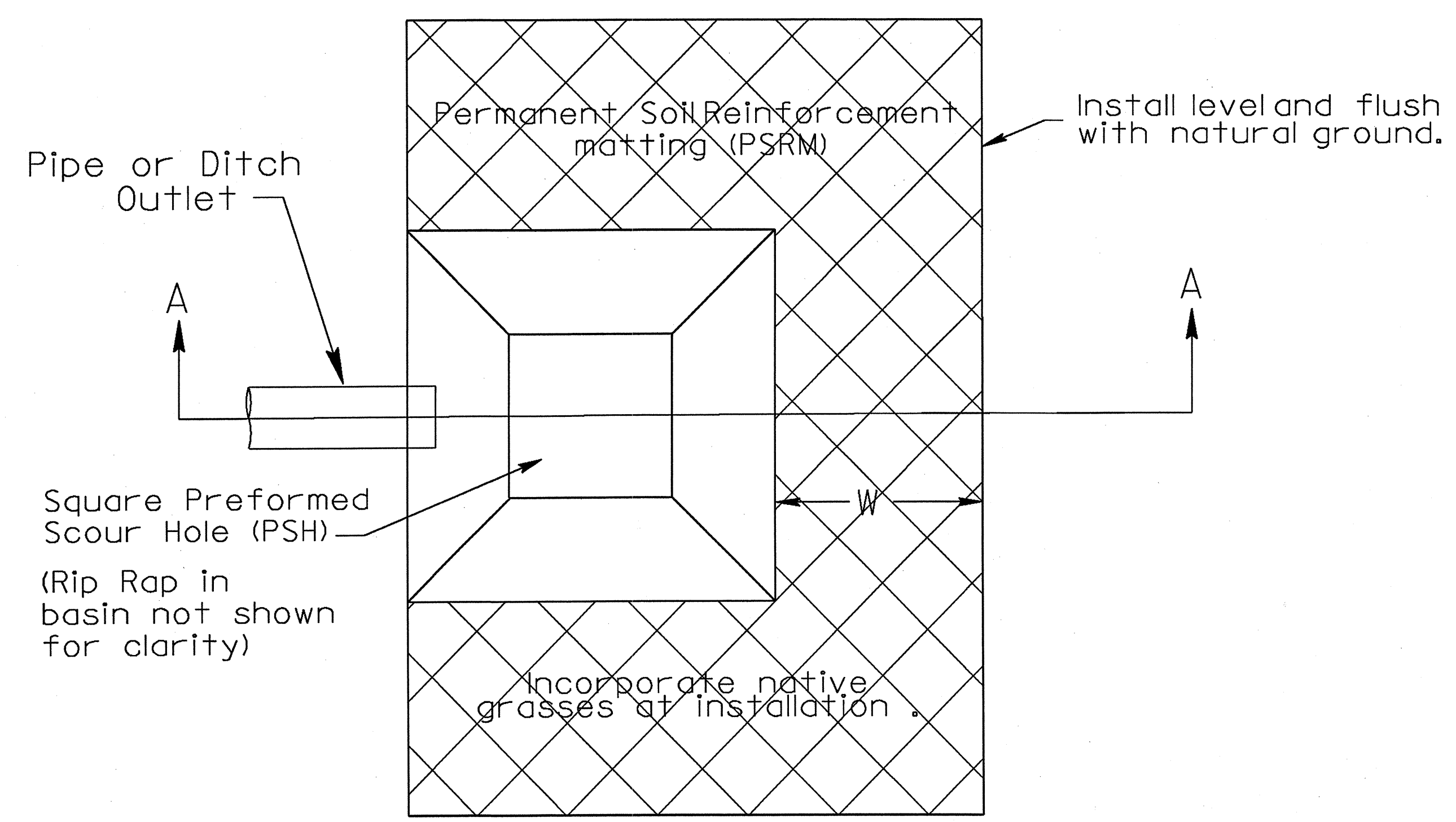
PLAN VIEW
