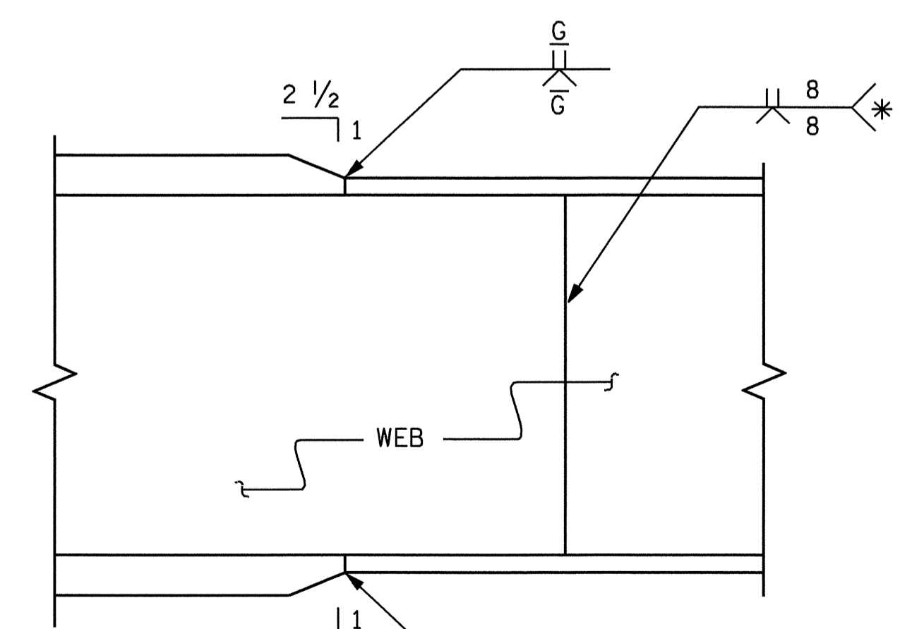
TYPICAL FLANGE AND WEB BUTT JOINT
