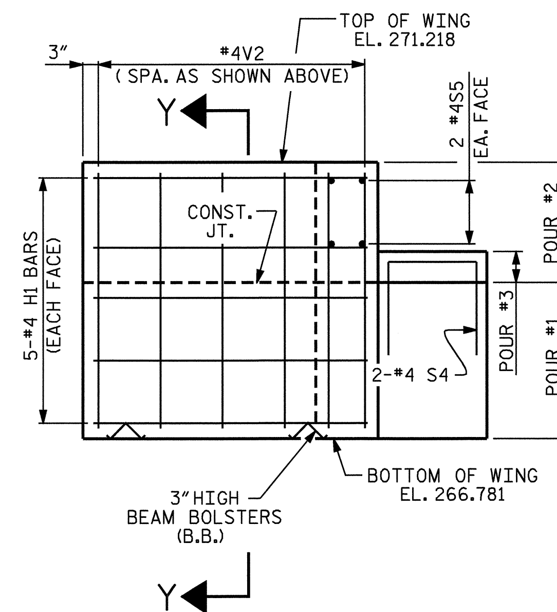
ELEVATION OF RIGHT WING (W2)
