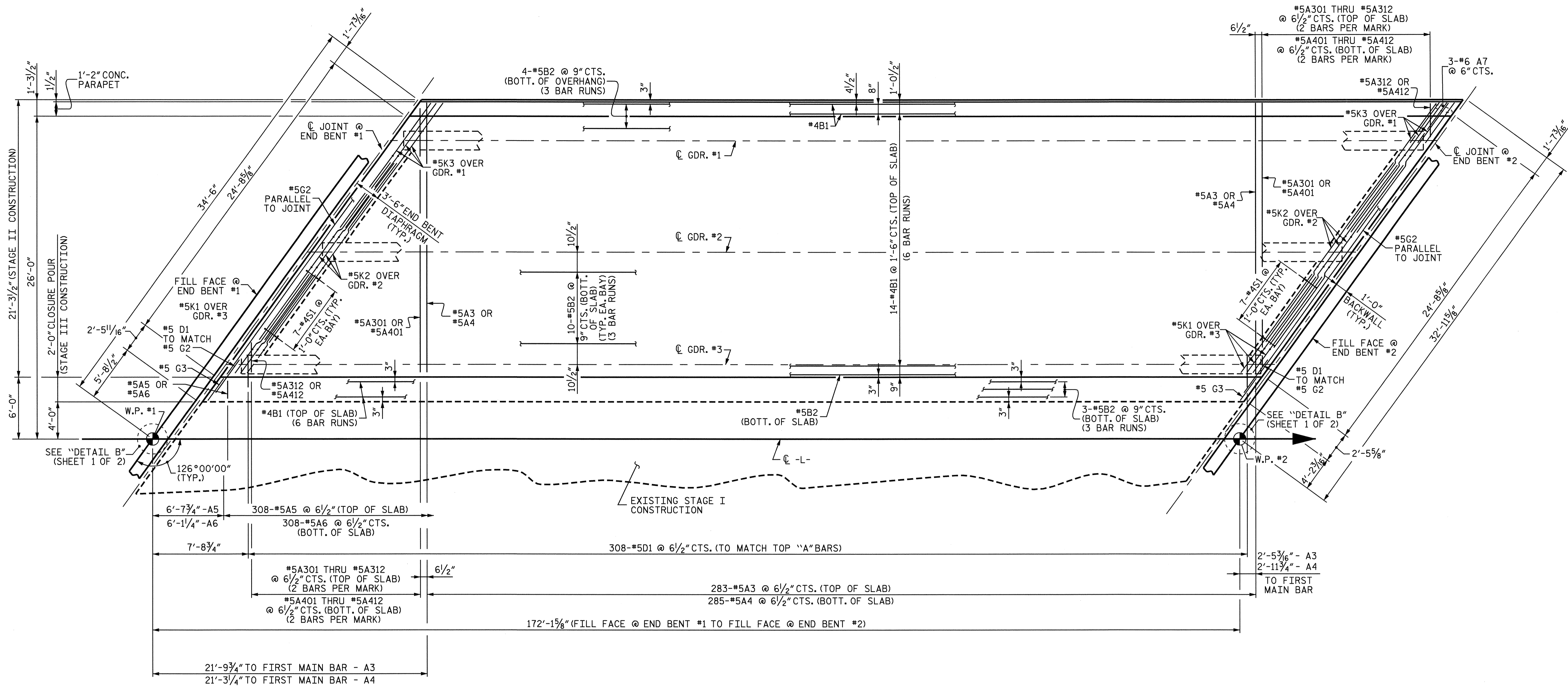
PLAN OF SPAN "A" (STAGE II & III CONSTRUCTION)
