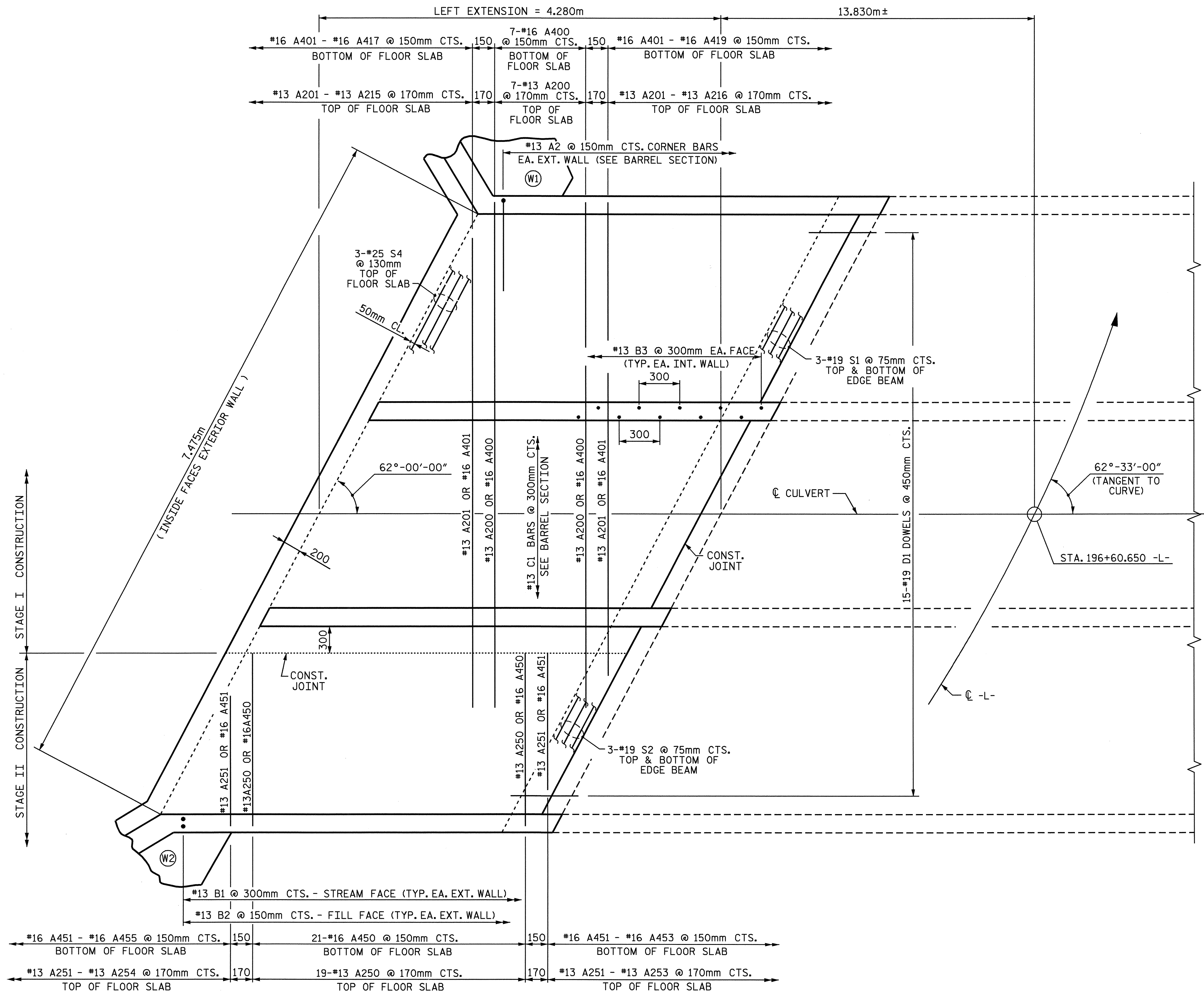
PLAN OF FLOOR SLAB
