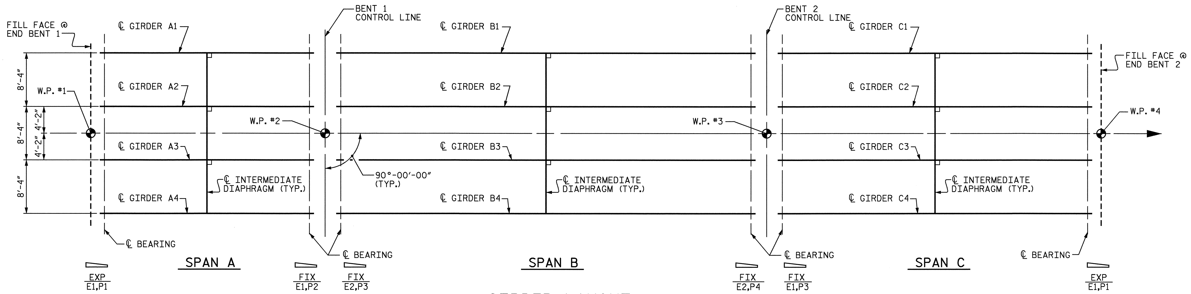
GIRDER LAYOUT INTERMEDIATE DIAPHRAGMS ARE LOCATED AT G GIRDER
