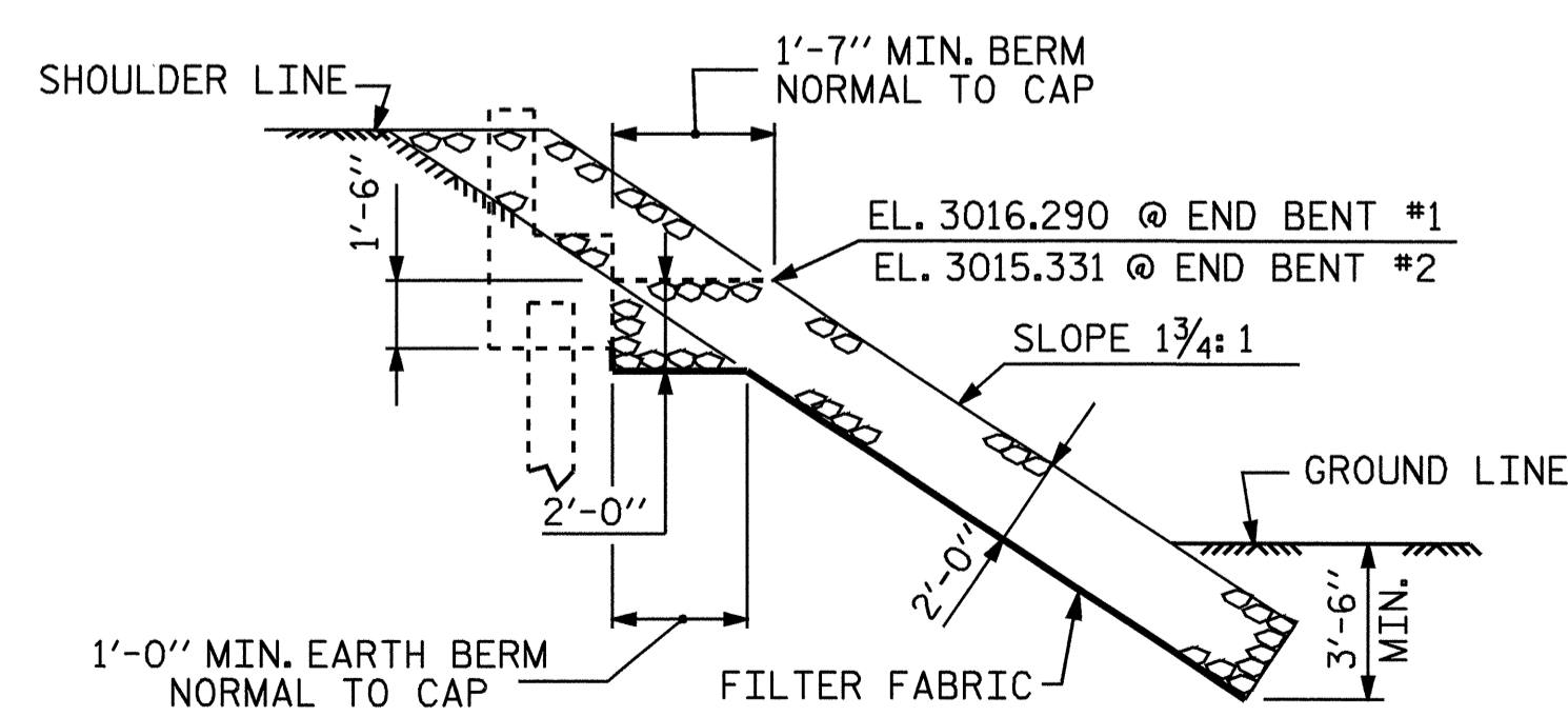
SECTION H-H
