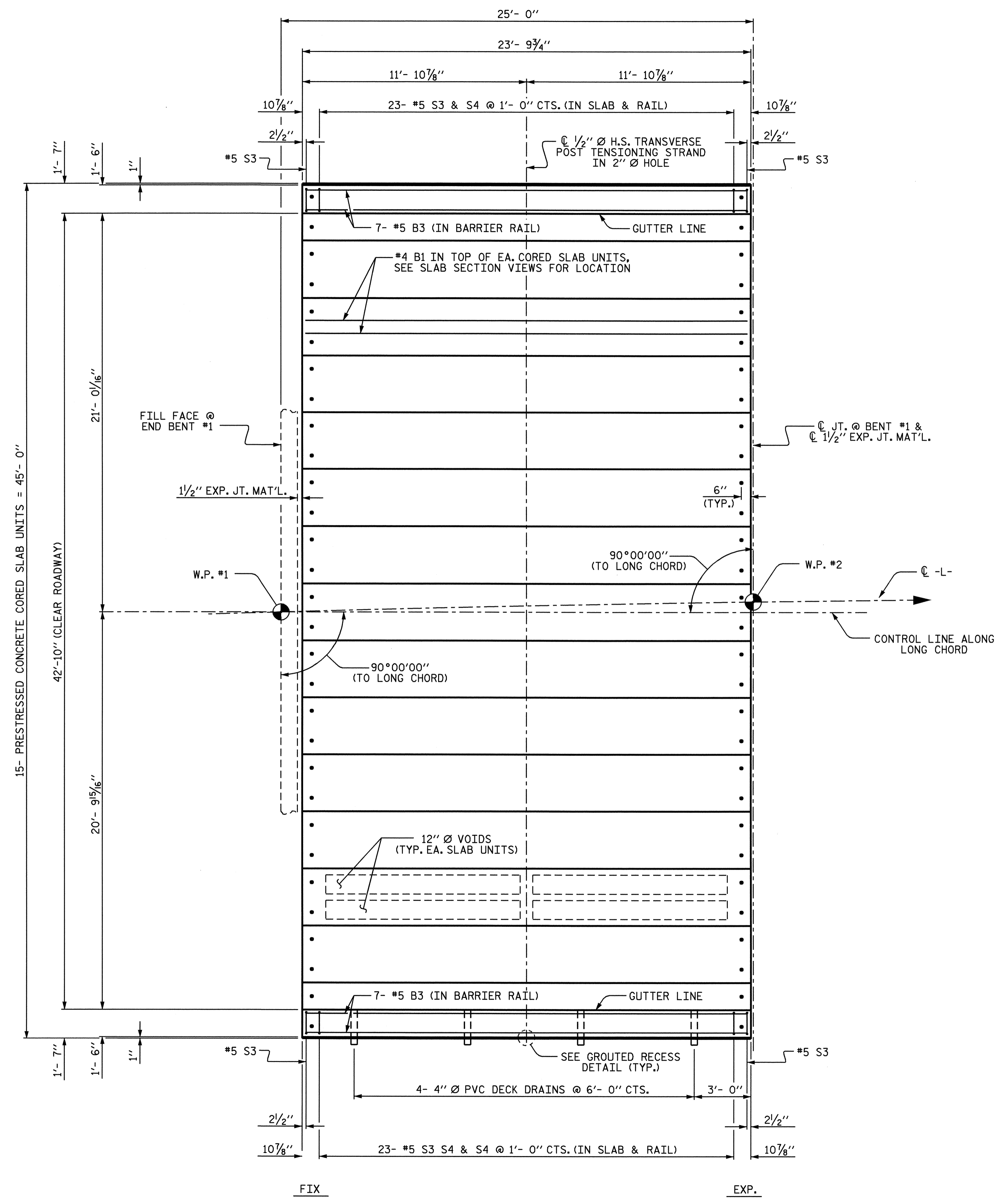
PLAN OF SPAN "A"
