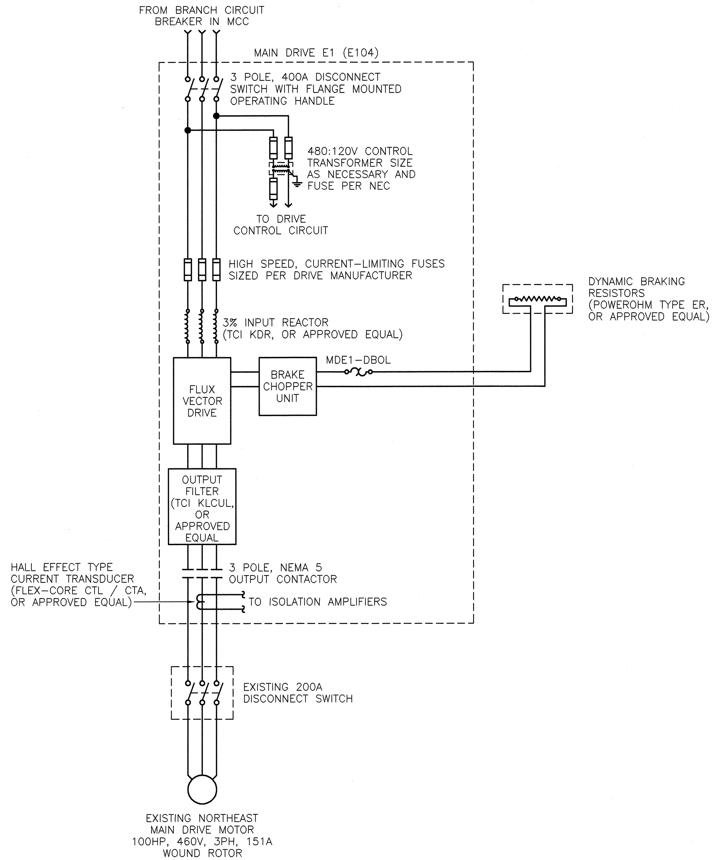
MAIN DRIVE POWER WIRING (DRIVE E1 SHOWN, DRIVE E2, W1 AND W2 SIMILAR)
