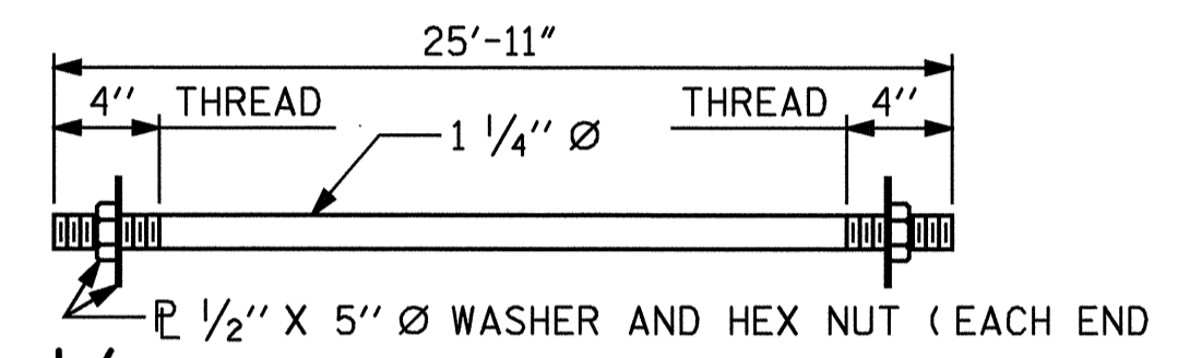
1 1/4" Ø TIE ROD ASSEMBLY
