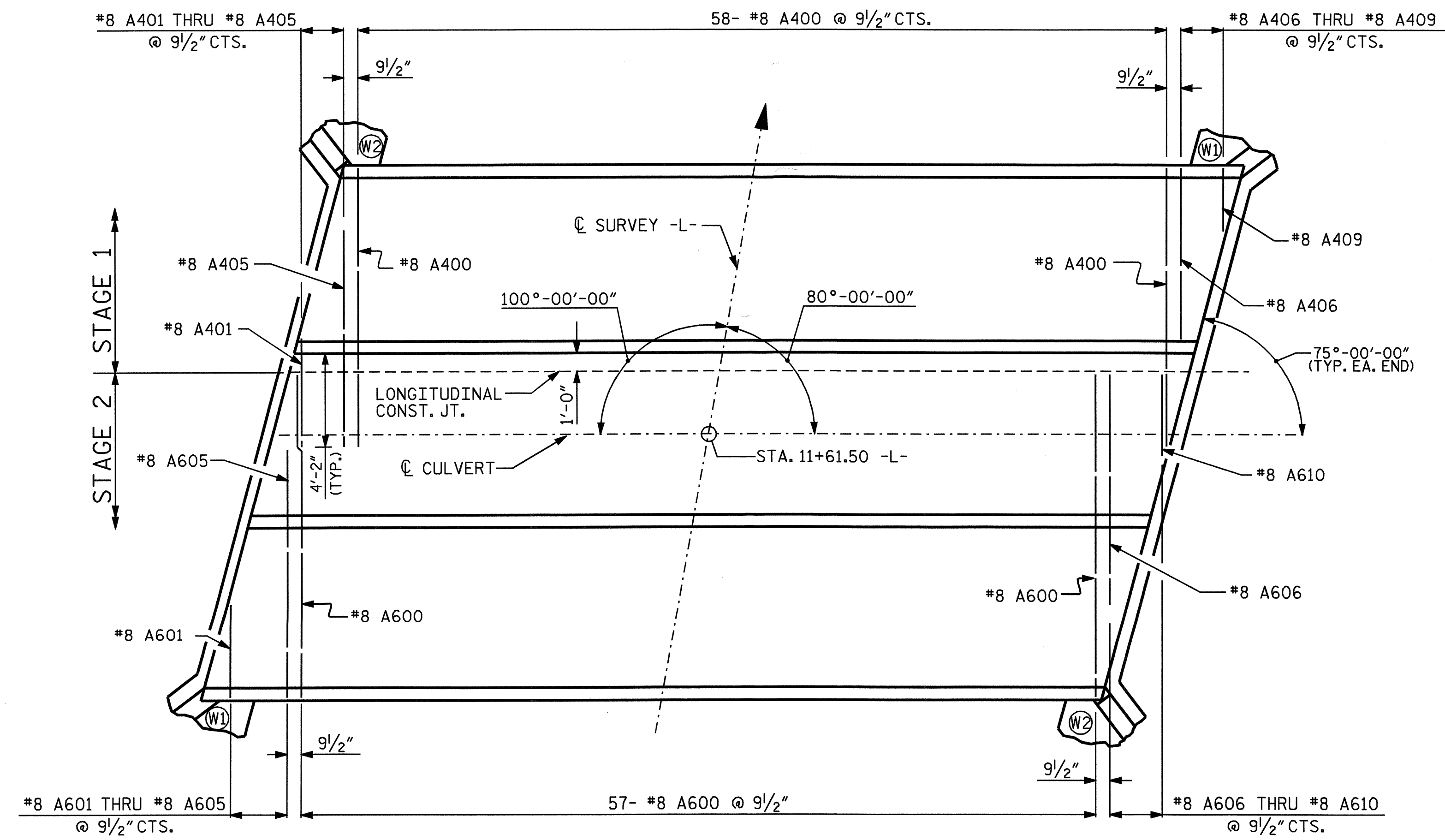
BOTTOM OF FLOOR SLAB-'A' BAR LAYOUT
