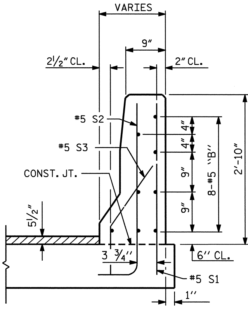
SECTION L-L
