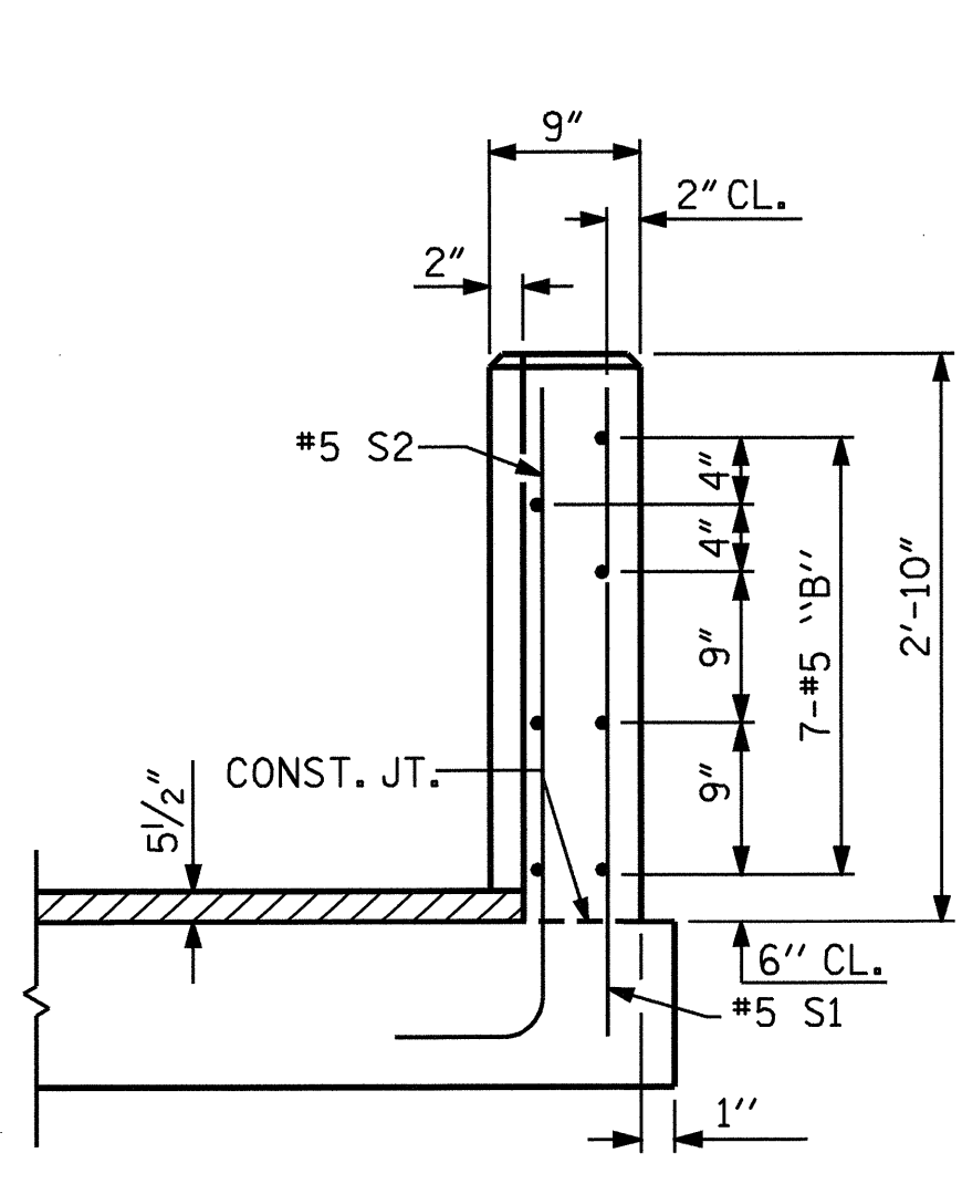
END VIEW
