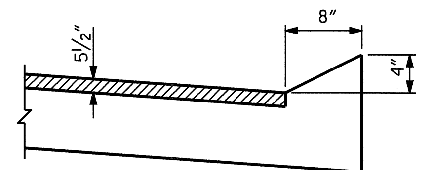
SECTION N-N
