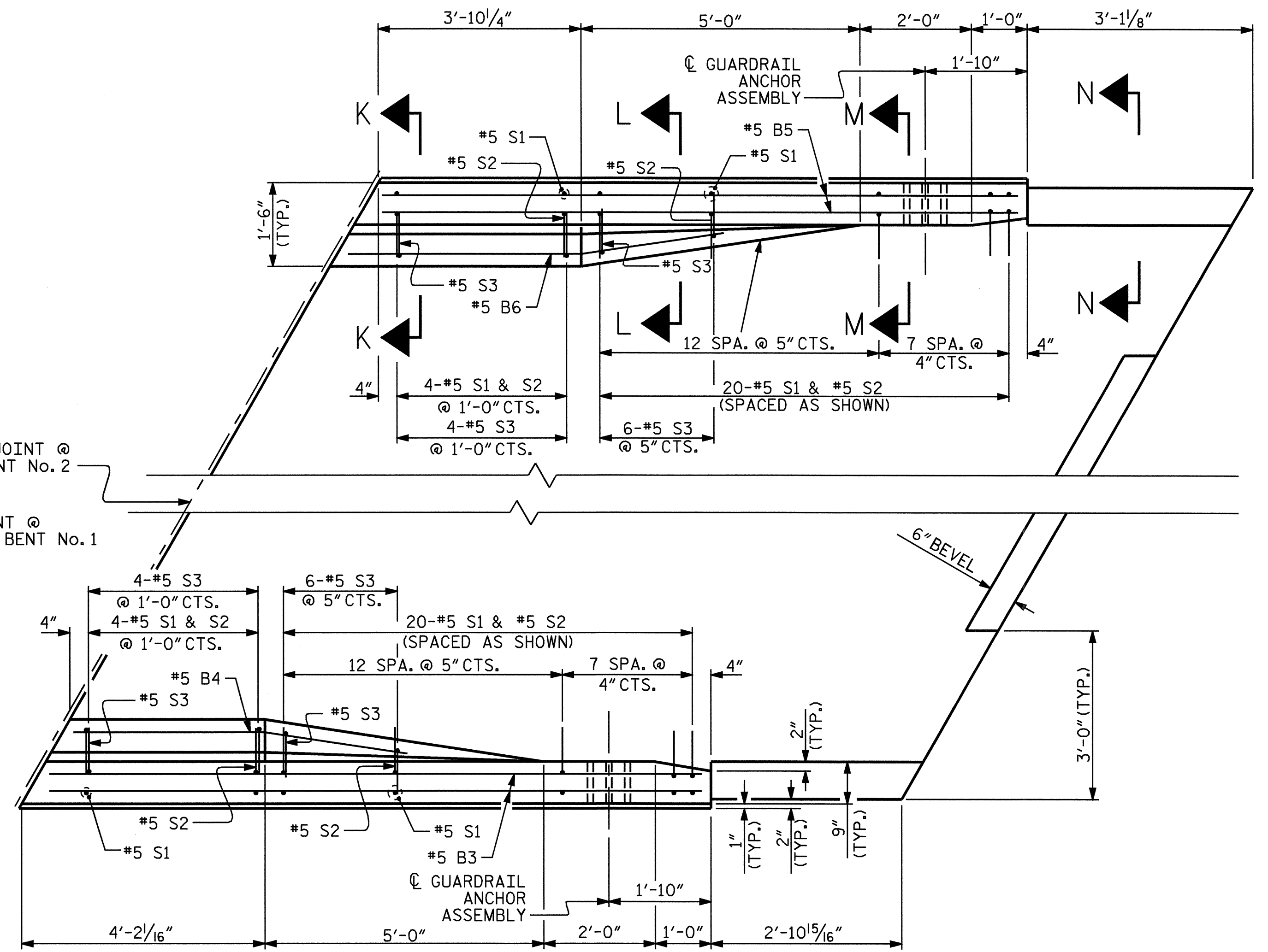
PLAN AT END BENT No. 2
