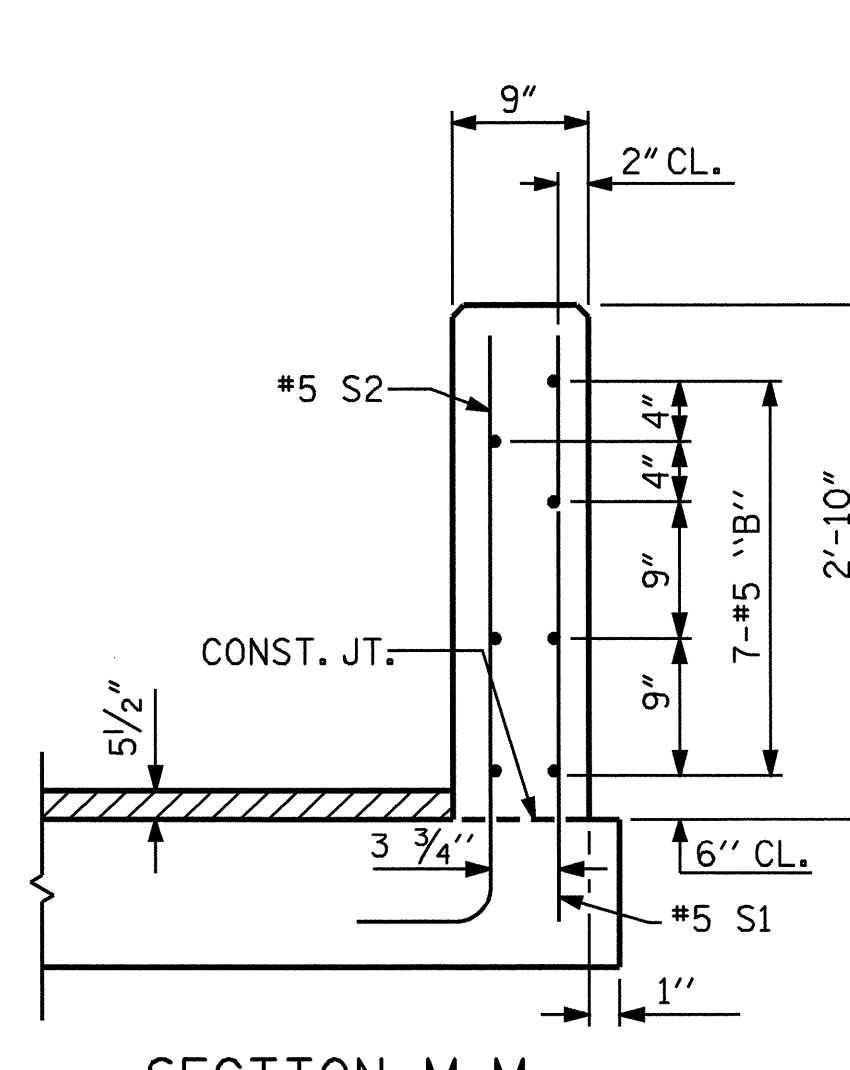
SECTION M-M
