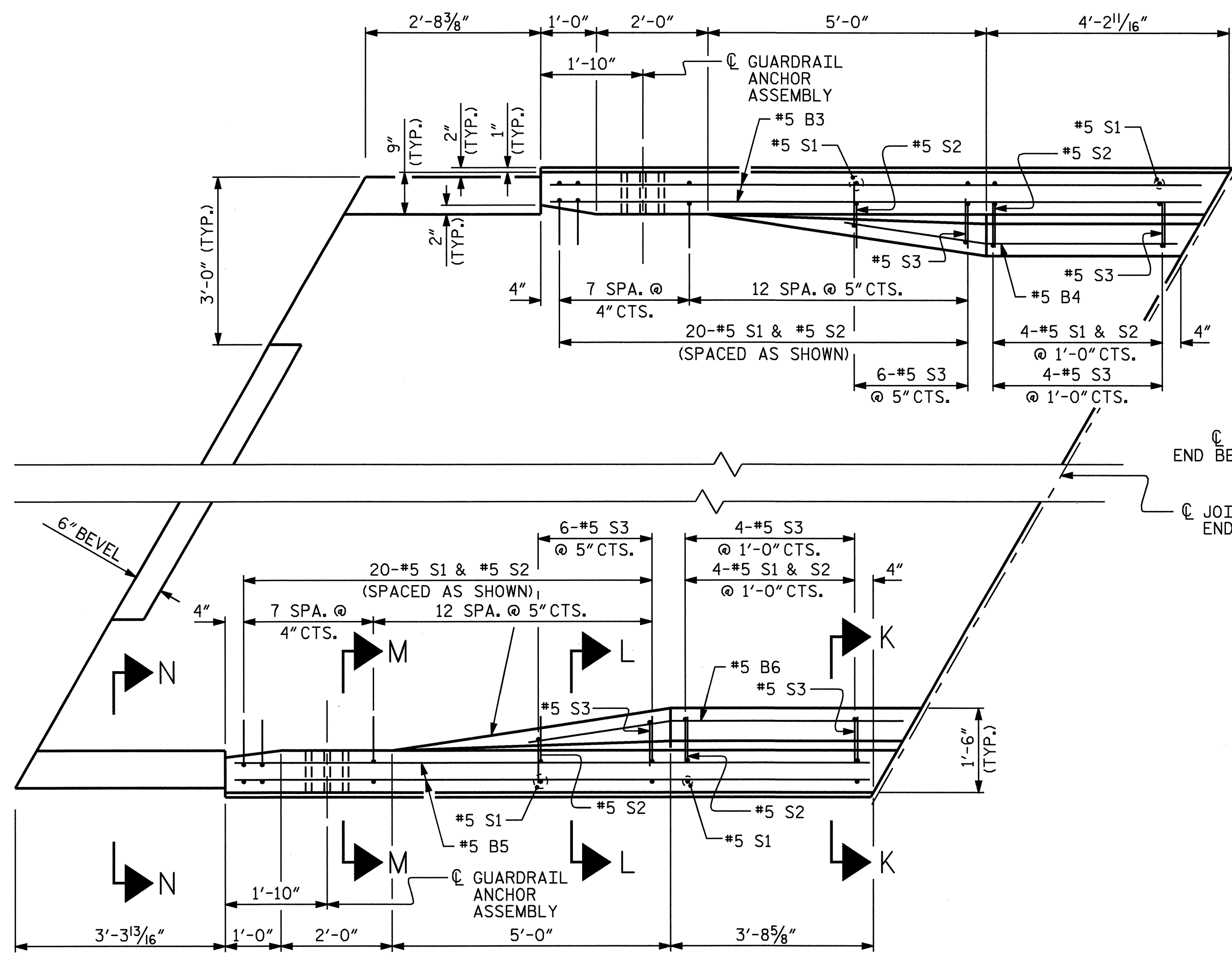
PLAN AT END BENT No. 1
