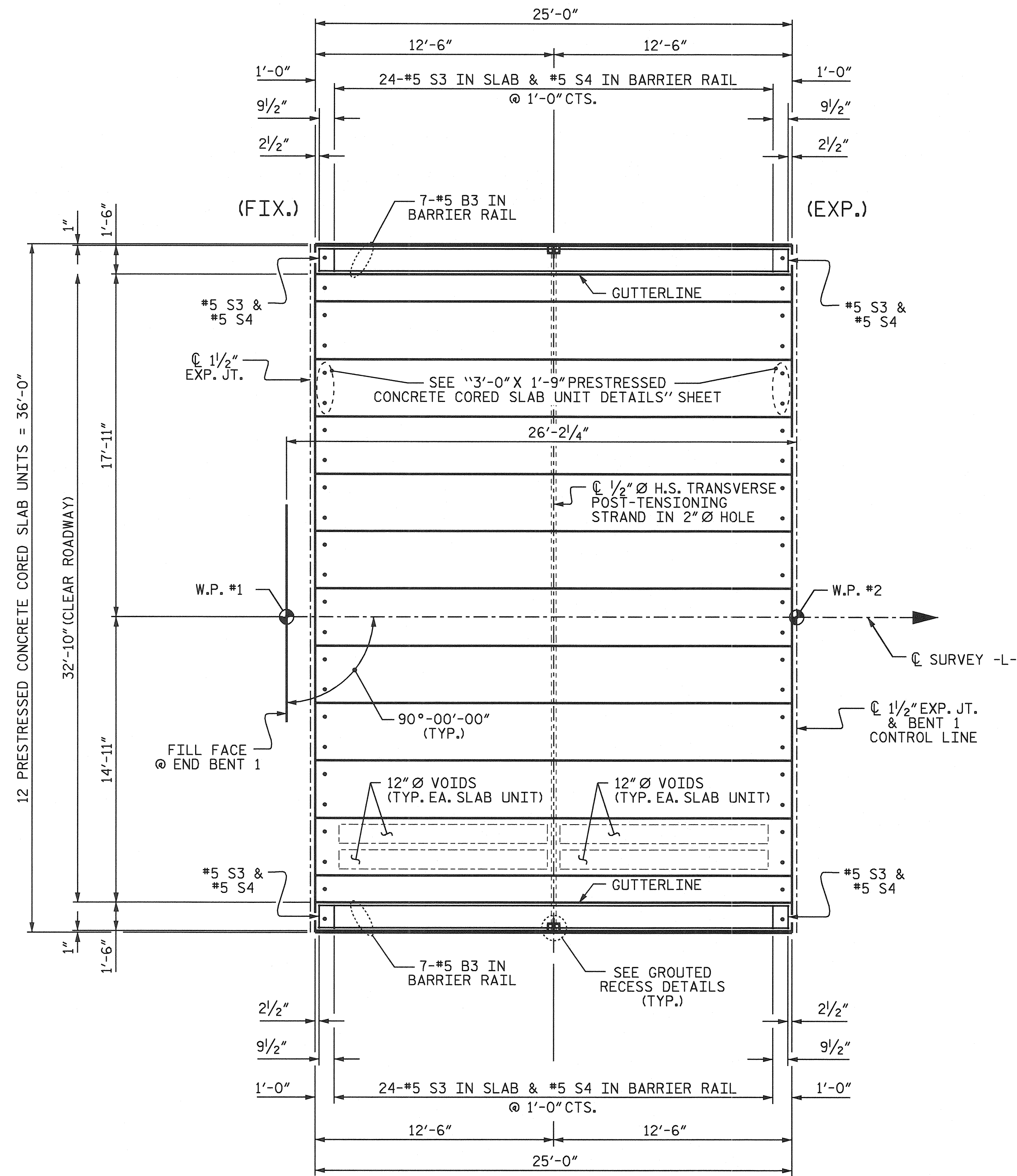
PLAN OF SPAN A
