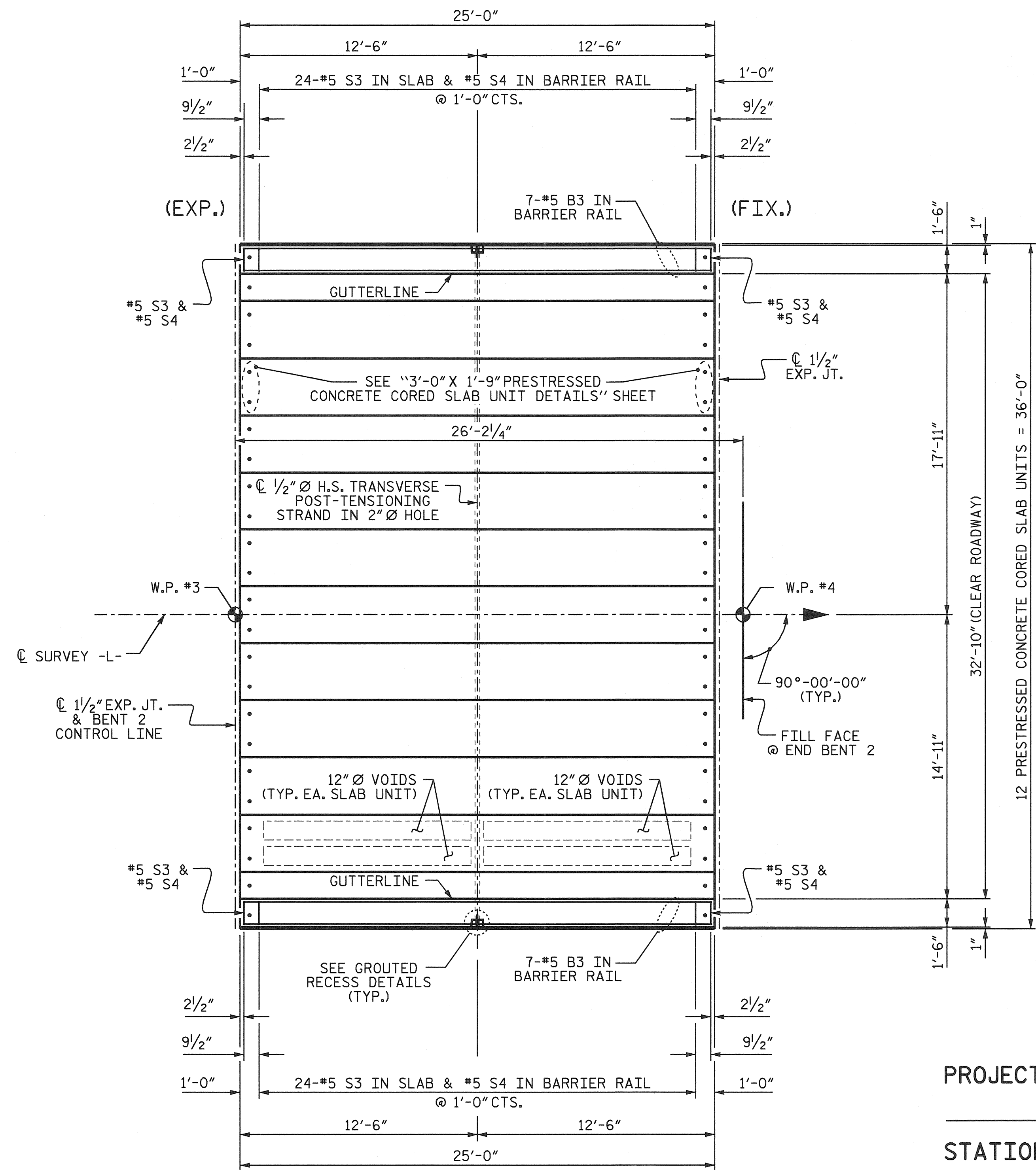
PLAN OF SPAN C
